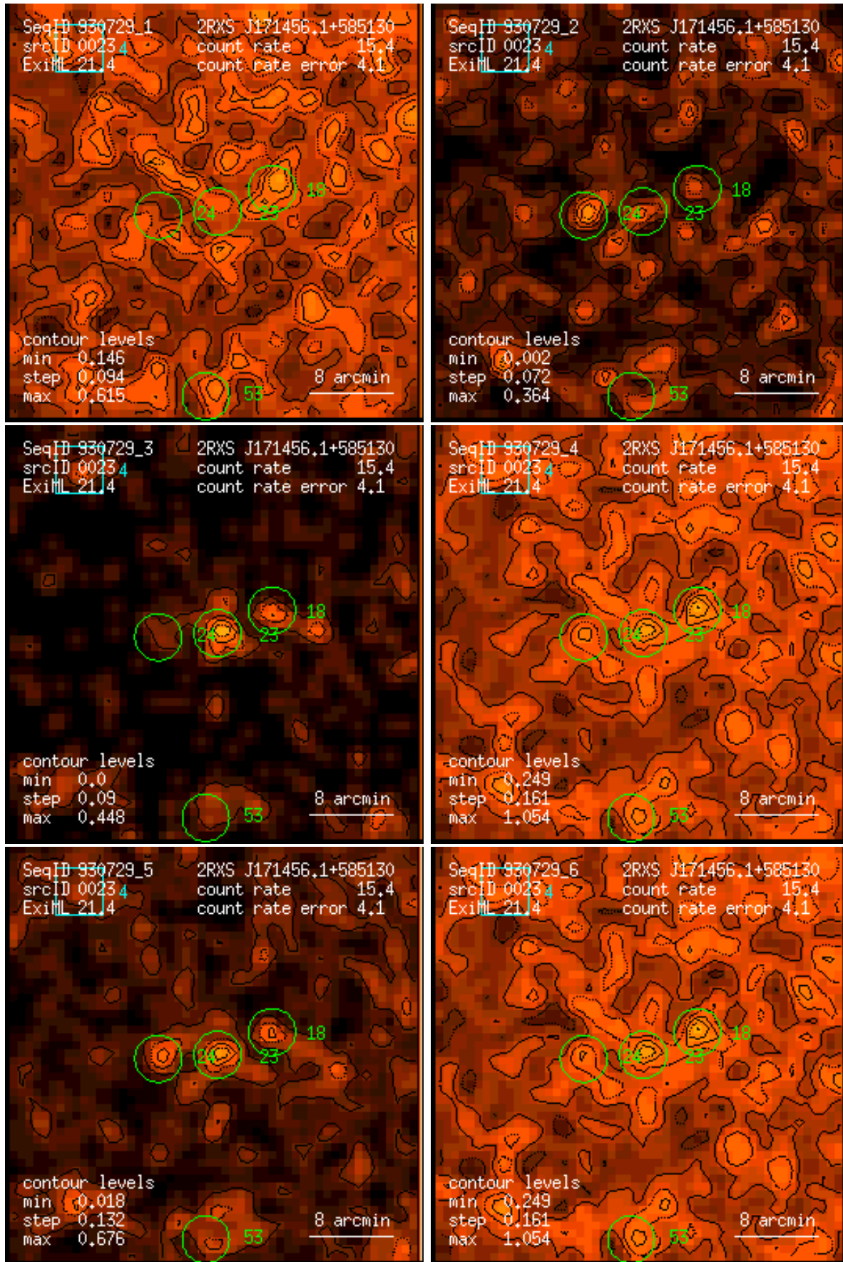
Figure 23: RASS 930729: detection 0023: band rate images, Gaussian filter: (1) PSPC channels 11 – 41, (2) 52 – 90, (3) 91 – 201, (4) 11 – 235, (5) 52 – 201, (6) 11 – 201. Broad band rates in counts/ks. Band rate contour levels in counts/ks/arcmin 2 .
