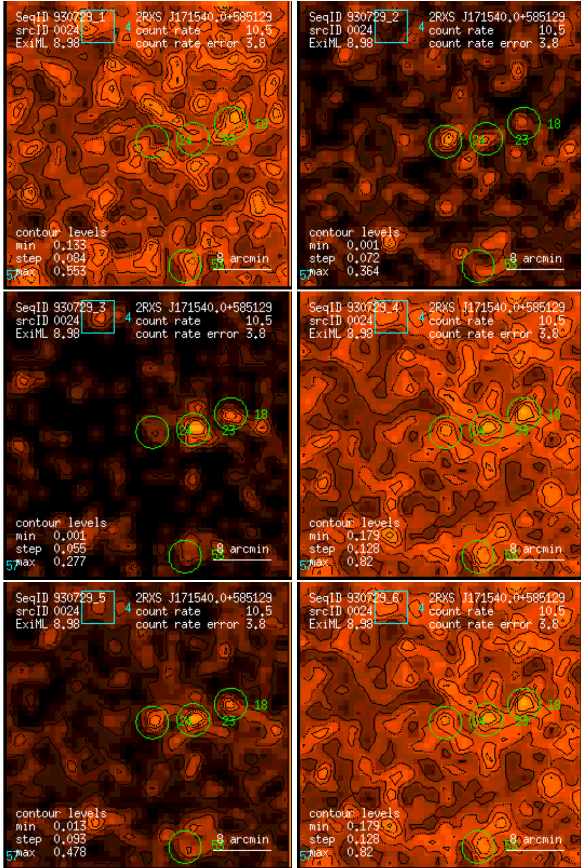
Figure 24: RASS 930729: detection 0024: band rate images, Gaussian filter: (1) PSPC channels 11 – 41, (2) 52 – 90, (3) 91 – 201, (4) 11 – 235, (5) 52 – 201, (6) 11 – 201. Broad band rates in counts/ks. Band rate contour levels in counts/ks/arcmin 2 .
