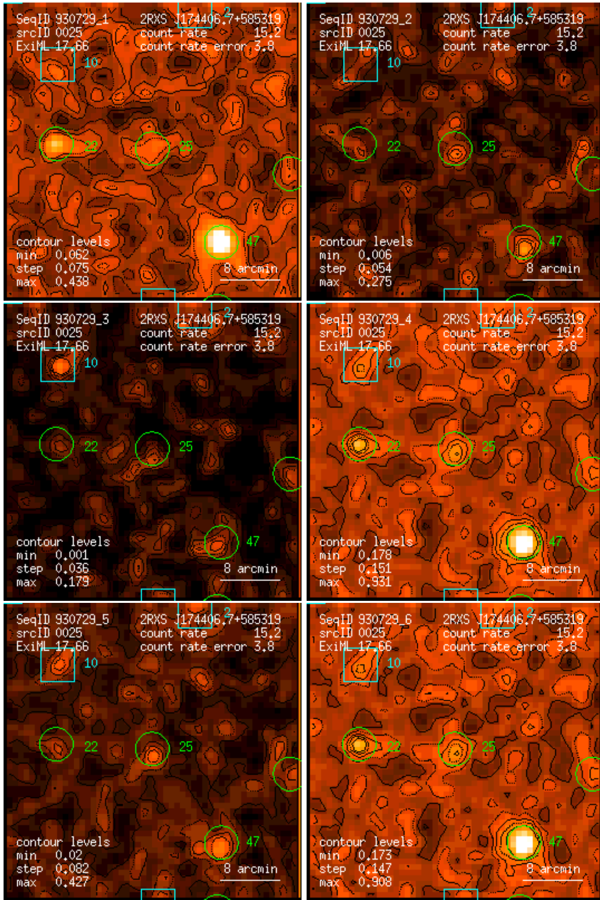
Figure 25: RASS 930729: detection 0025: band rate images, Gaussian filter: (1) PSPC channels 11 – 41, (2) 52 – 90, (3) 91 – 201, (4) 11 – 235, (5) 52 – 201, (6) 11 – 201. Broad band rates in counts/ks. Band rate contour levels in counts/ks/arcmin 2 .
