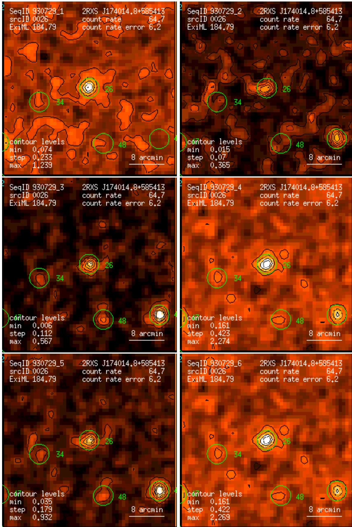
Figure 26: RASS 930729: detection 0026: band rate images, Gaussian filter: (1) PSPC channels 11 – 41, (2) 52 – 90, (3) 91 – 201, (4) 11 – 235, (5) 52 – 201, (6) 11 – 201. Broad band rates in counts/ks. Band rate contour levels in counts/ks/arcmin 2 .
