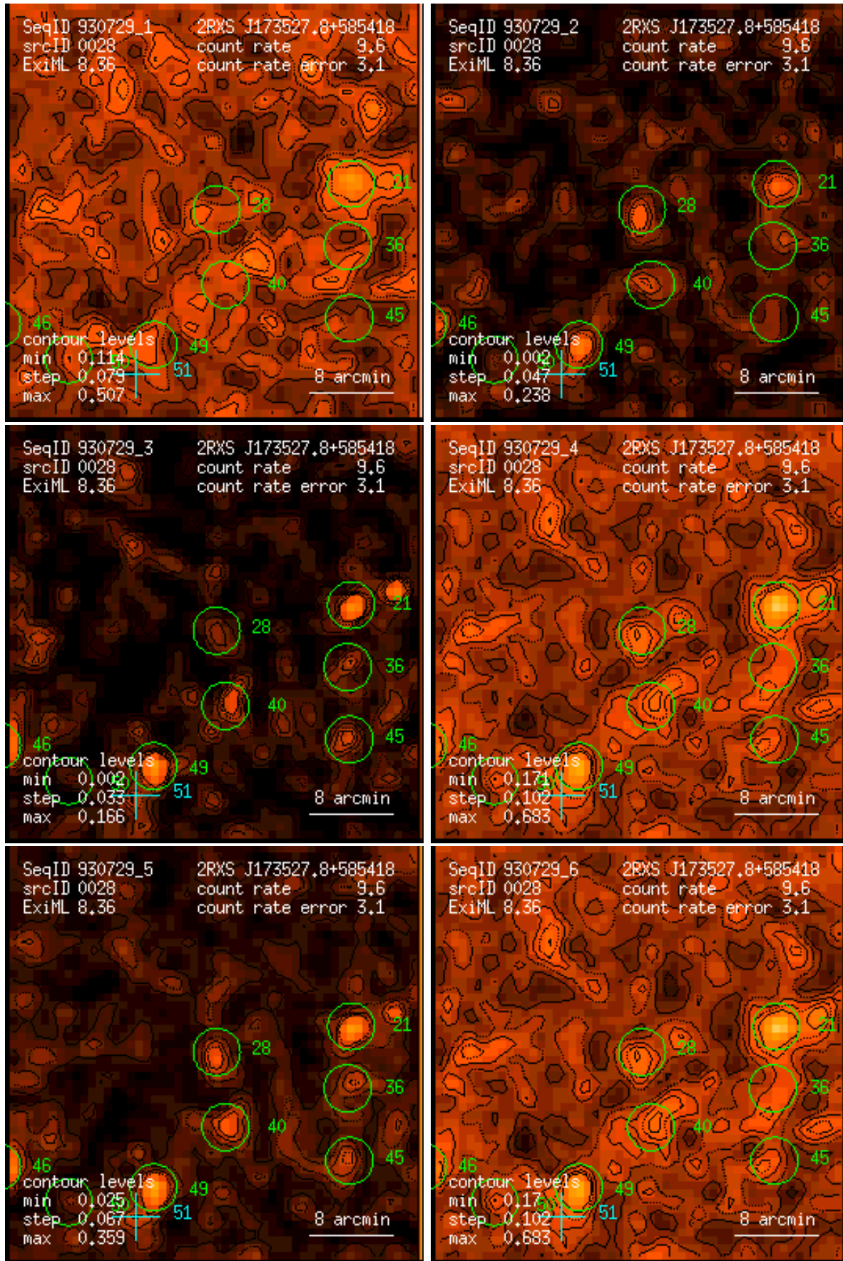
Figure 28: RASS 930729: detection 0028: band rate images, Gaussian filter: (1) PSPC channels 11 – 41, (2) 52 – 90, (3) 91 – 201, (4) 11 – 235, (5) 52 – 201, (6) 11 – 201. Broad band rates in counts/ks. Band rate contour levels in counts/ks/arcmin 2 .
