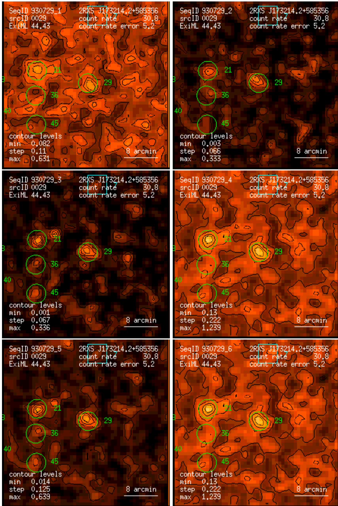
Figure 29: RASS 930729: detection 0029: band rate images, Gaussian filter: (1) PSPC channels 11 – 41, (2) 52 – 90, (3) 91 – 201, (4) 11 – 235, (5) 52 – 201, (6) 11 – 201. Broad band rates in counts/ks. Band rate contour levels in counts/ks/arcmin 2 .
