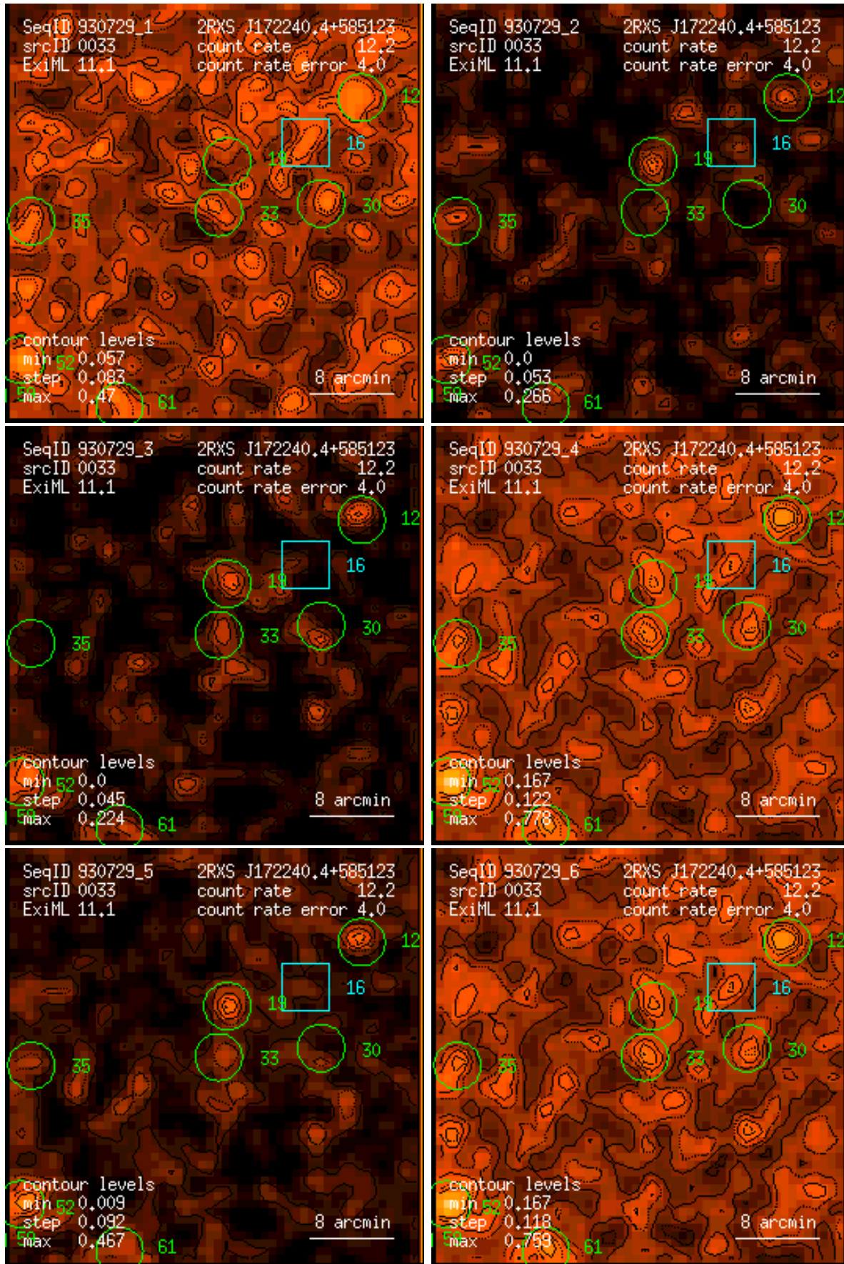
Figure 33: RASS 930729: detection 0033: band rate images, Gaussian filter: (1) PSPC channels 11 – 41, (2) 52 – 90, (3) 91 – 201, (4) 11 – 235, (5) 52 – 201, (6) 11 – 201. Broad band rates in counts/ks. Band rate contour levels in counts/ks/arcmin 2 .
