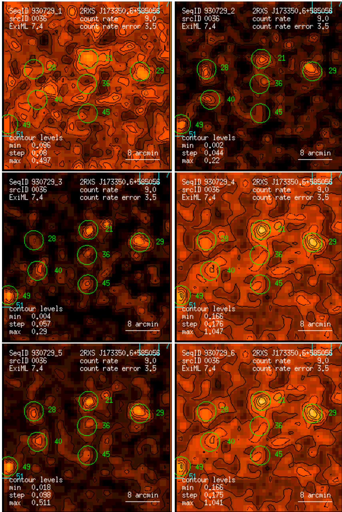
Figure 36: RASS 930729: detection 0036: band rate images, Gaussian filter: (1) PSPC channels 11 – 41, (2) 52 – 90, (3) 91 – 201, (4) 11 – 235, (5) 52 – 201, (6) 11 – 201. Broad band rates in counts/ks. Band rate contour levels in counts/ks/arcmin 2 .
