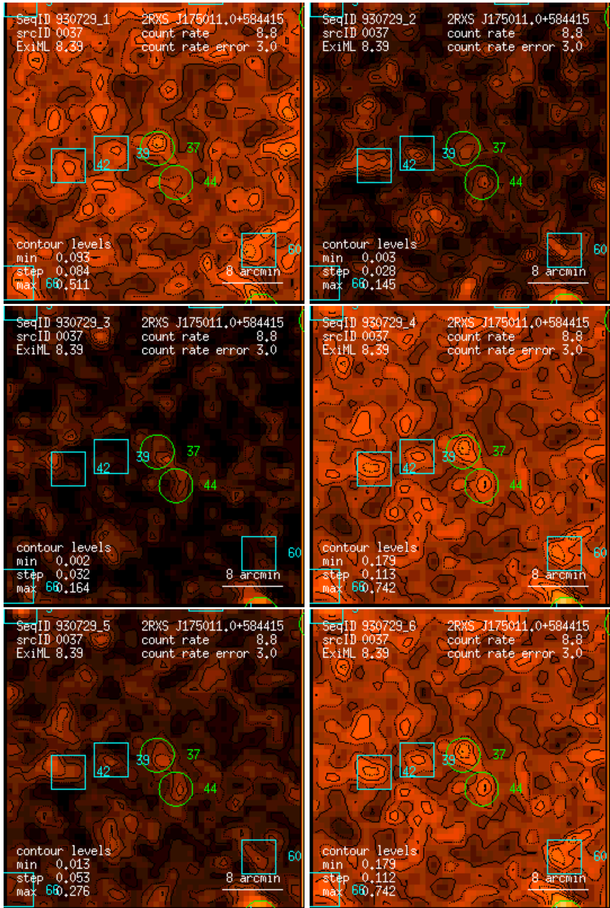
Figure 37: RASS 930729: detection 0037: band rate images, Gaussian filter: (1) PSPC channels 11 – 41, (2) 52 – 90, (3) 91 – 201, (4) 11 – 235, (5) 52 – 201, (6) 11 – 201. Broad band rates in counts/ks. Band rate contour levels in counts/ks/arcmin 2 .
