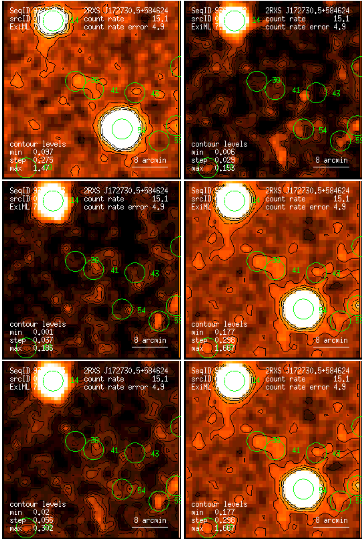
Figure 41: RASS 930729: detection 0041: band rate images, Gaussian filter: (1) PSPC channels 11 – 41, (2) 52 – 90, (3) 91 – 201, (4) 11 – 235, (5) 52 – 201, (6) 11 – 201. Broad band rates in counts/ks. Band rate contour levels in counts/ks/arcmin 2 .
