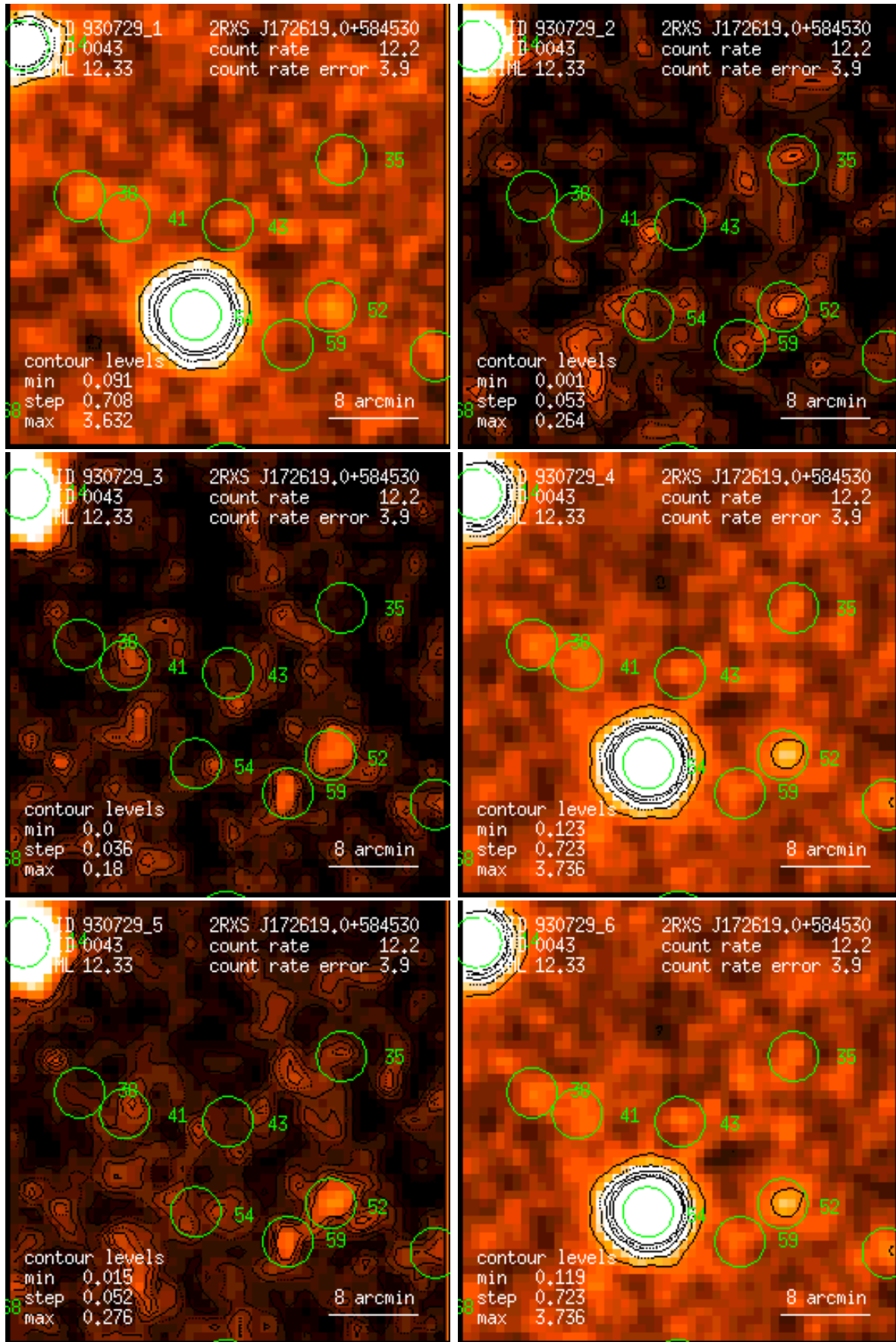
Figure 43: RASS 930729: detection 0043: band rate images, Gaussian filter: (1) PSPC channels 11 – 41, (2) 52 – 90, (3) 91 – 201, (4) 11 – 235, (5) 52 – 201, (6) 11 – 201. Broad band rates in counts/ks. Band rate contour levels in counts/ks/arcmin 2 .
