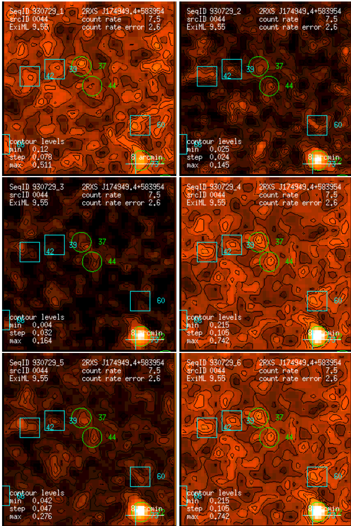
Figure 44: RASS 930729: detection 0044: band rate images, Gaussian filter: (1) PSPC channels 11 – 41, (2) 52 – 90, (3) 91 – 201, (4) 11 – 235, (5) 52 – 201, (6) 11 – 201. Broad band rates in counts/ks. Band rate contour levels in counts/ks/arcmin 2 .
