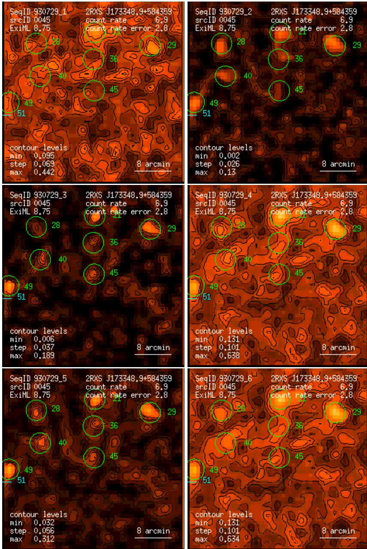
Figure 45: RASS 930729: detection 0045: band rate images, Gaussian filter: (1) PSPC channels 11 – 41, (2) 52 – 90, (3) 91 – 201, (4) 11 – 235, (5) 52 – 201, (6) 11 – 201. Broad band rates in counts/ks. Band rate contour levels in counts/ks/arcmin 2 .
