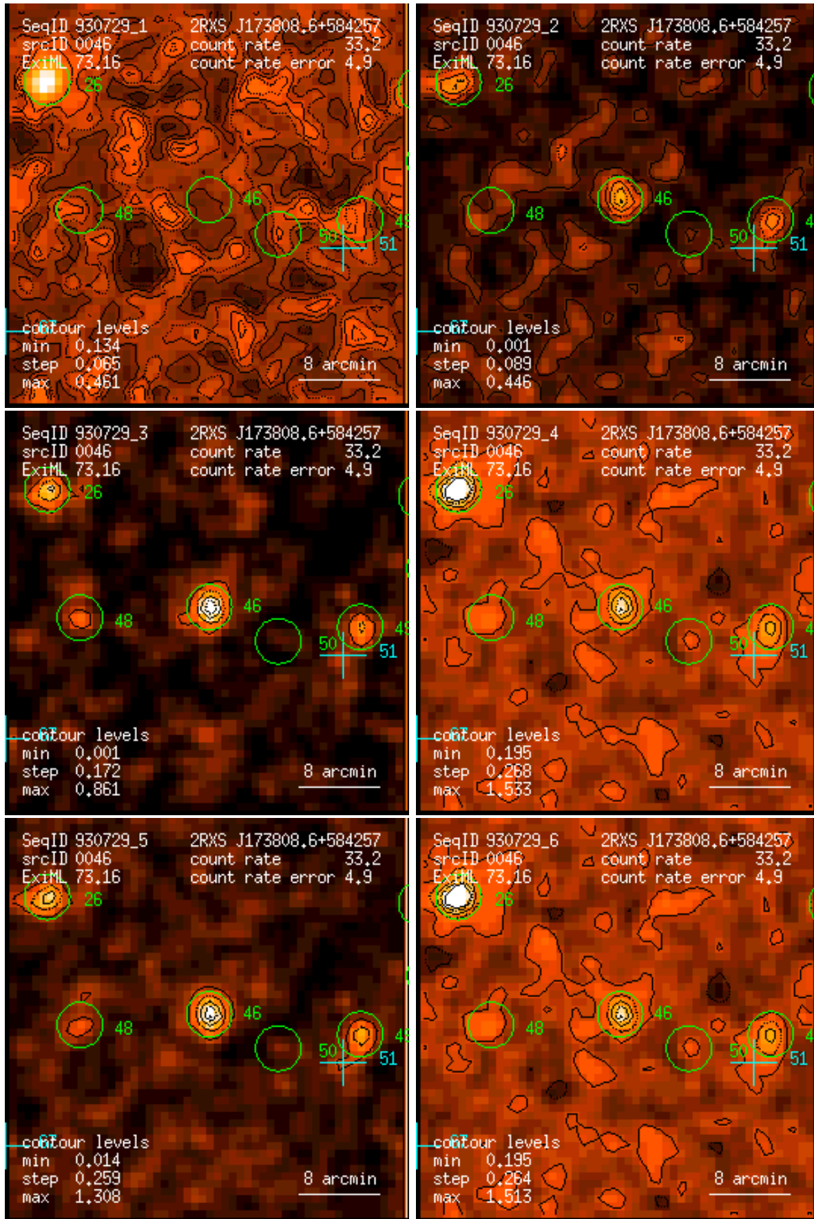
Figure 46: RASS 930729: detection 0046: band rate images, Gaussian filter: (1) PSPC channels 11 – 41, (2) 52 – 90, (3) 91 – 201, (4) 11 – 235, (5) 52 – 201, (6) 11 – 201. Broad band rates in counts/ks. Band rate contour levels in counts/ks/arcmin 2 .
