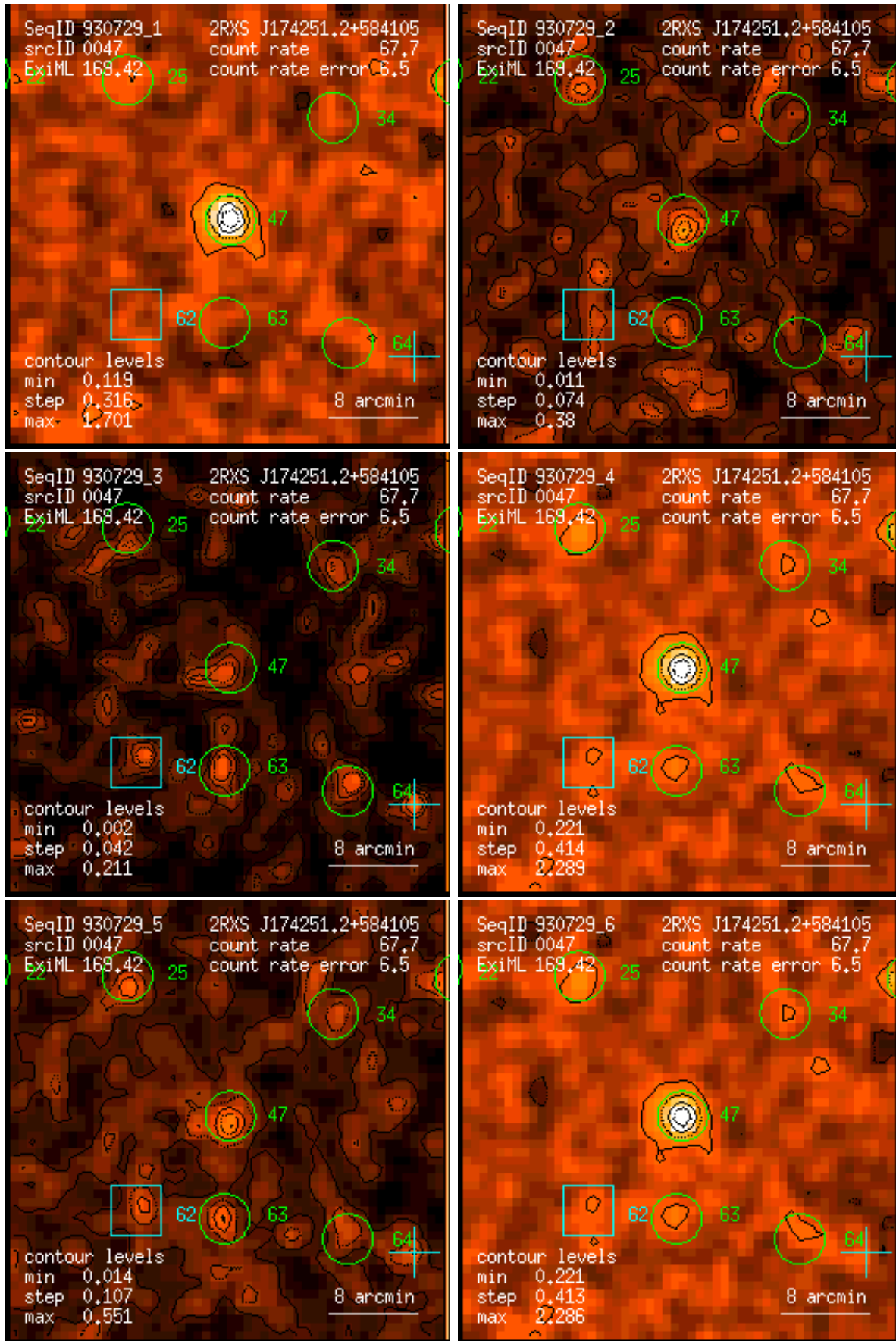
Figure 47: RASS 930729: detection 0047: band rate images, Gaussian filter: (1) PSPC channels 11 – 41, (2) 52 – 90, (3) 91 – 201, (4) 11 – 235, (5) 52 – 201, (6) 11 – 201. Broad band rates in counts/ks. Band rate contour levels in counts/ks/arcmin 2 .
