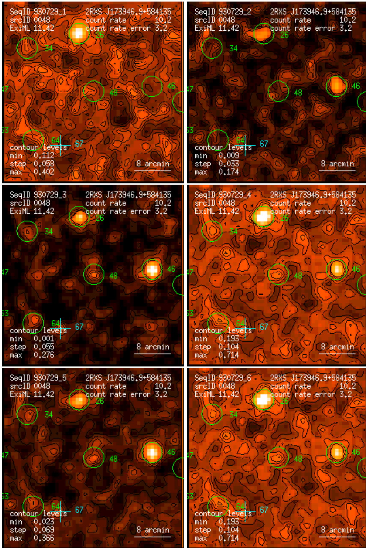
Figure 48: RASS 930729: detection 0048: band rate images, Gaussian filter: (1) PSPC channels 11 – 41, (2) 52 – 90, (3) 91 – 201, (4) 11 – 235, (5) 52 – 201, (6) 11 – 201. Broad band rates in counts/ks. Band rate contour levels in counts/ks/arcmin 2 .
