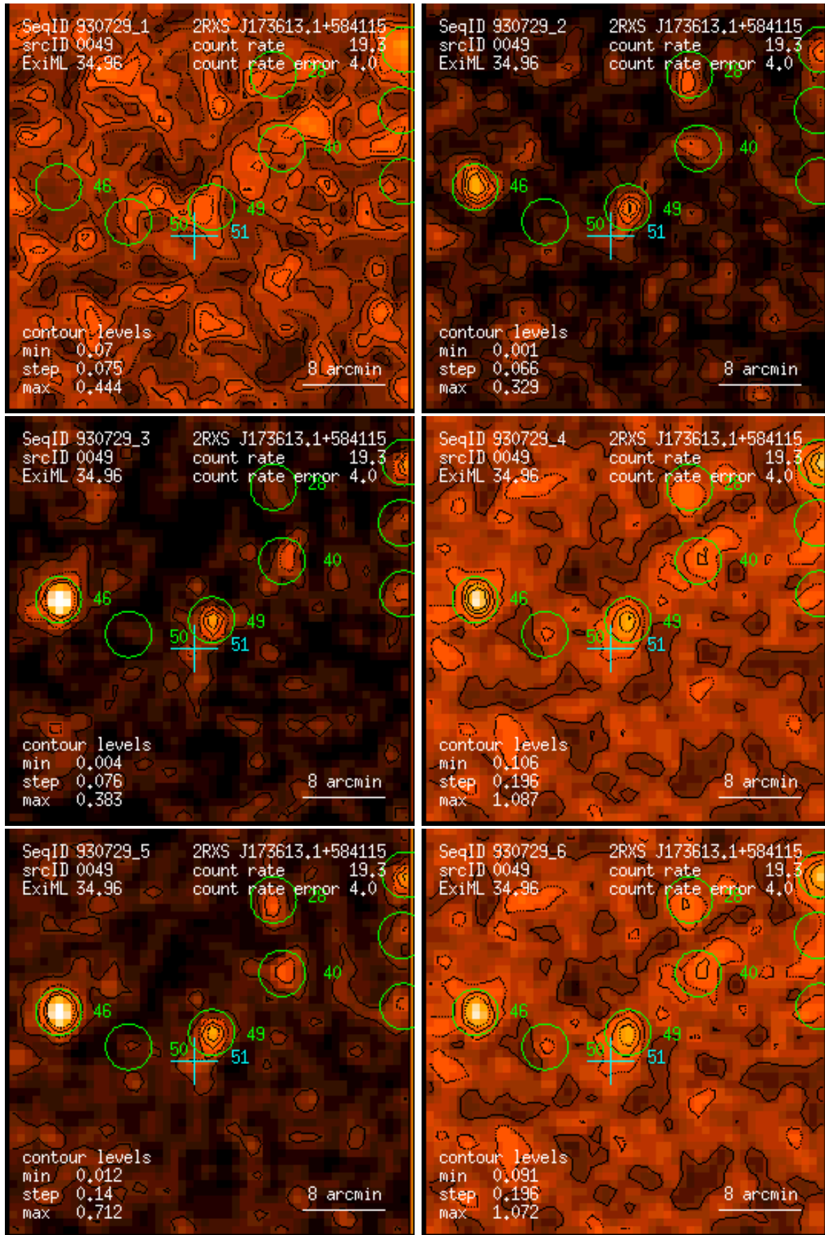
Figure 49: RASS 930729: detection 0049: band rate images, Gaussian filter: (1) PSPC channels 11 – 41, (2) 52 – 90, (3) 91 – 201, (4) 11 – 235, (5) 52 – 201, (6) 11 – 201. Broad band rates in counts/ks. Band rate contour levels in counts/ks/arcmin 2 .
