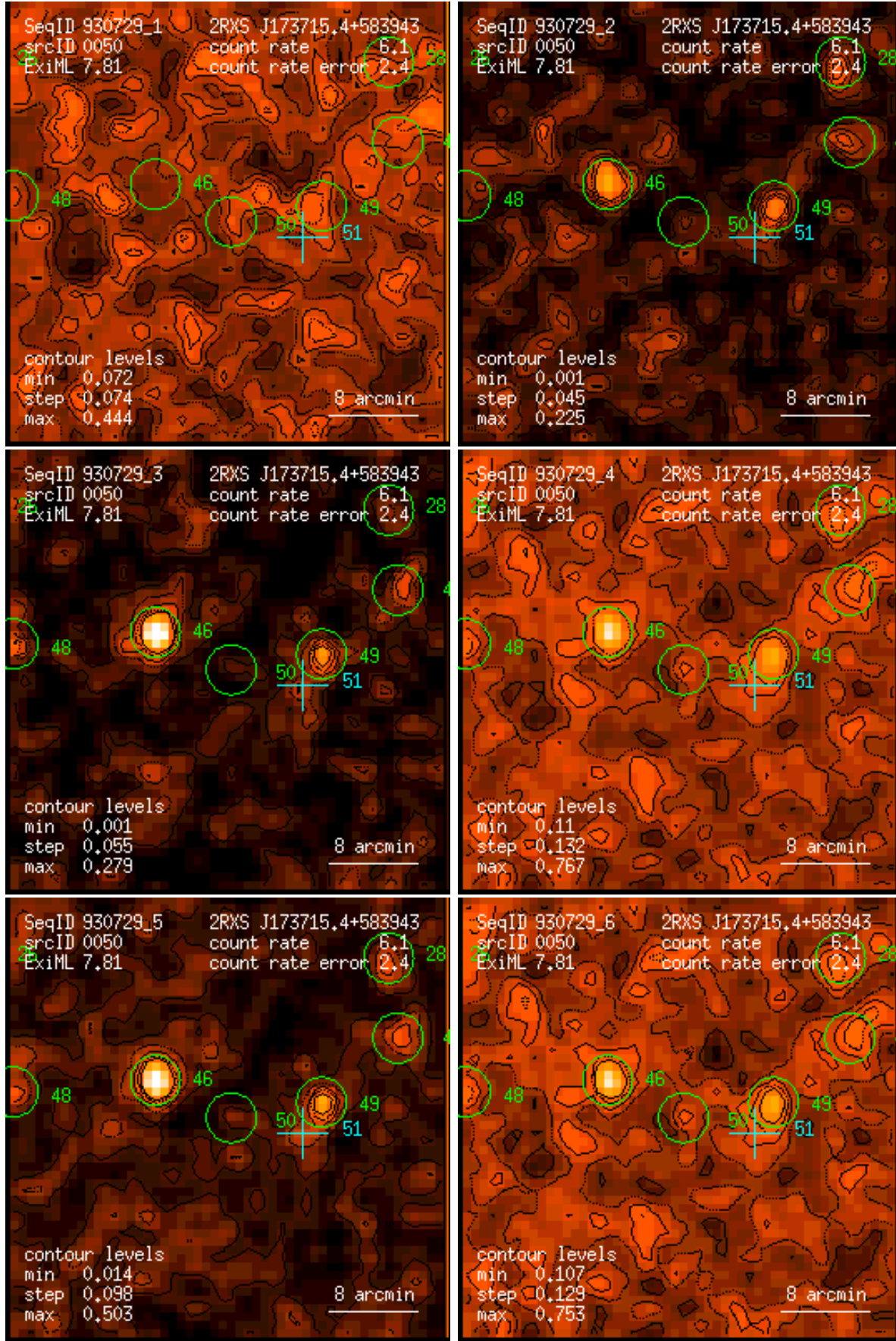
Figure 50: RASS 930729: detection 0050: band rate images, Gaussian filter: (1) PSPC channels 11 – 41, (2) 52 – 90, (3) 91 – 201, (4) 11 – 235, (5) 52 – 201, (6) 11 – 201. Broad band rates in counts/ks. Band rate contour levels in counts/ks/arcmin 2 .
