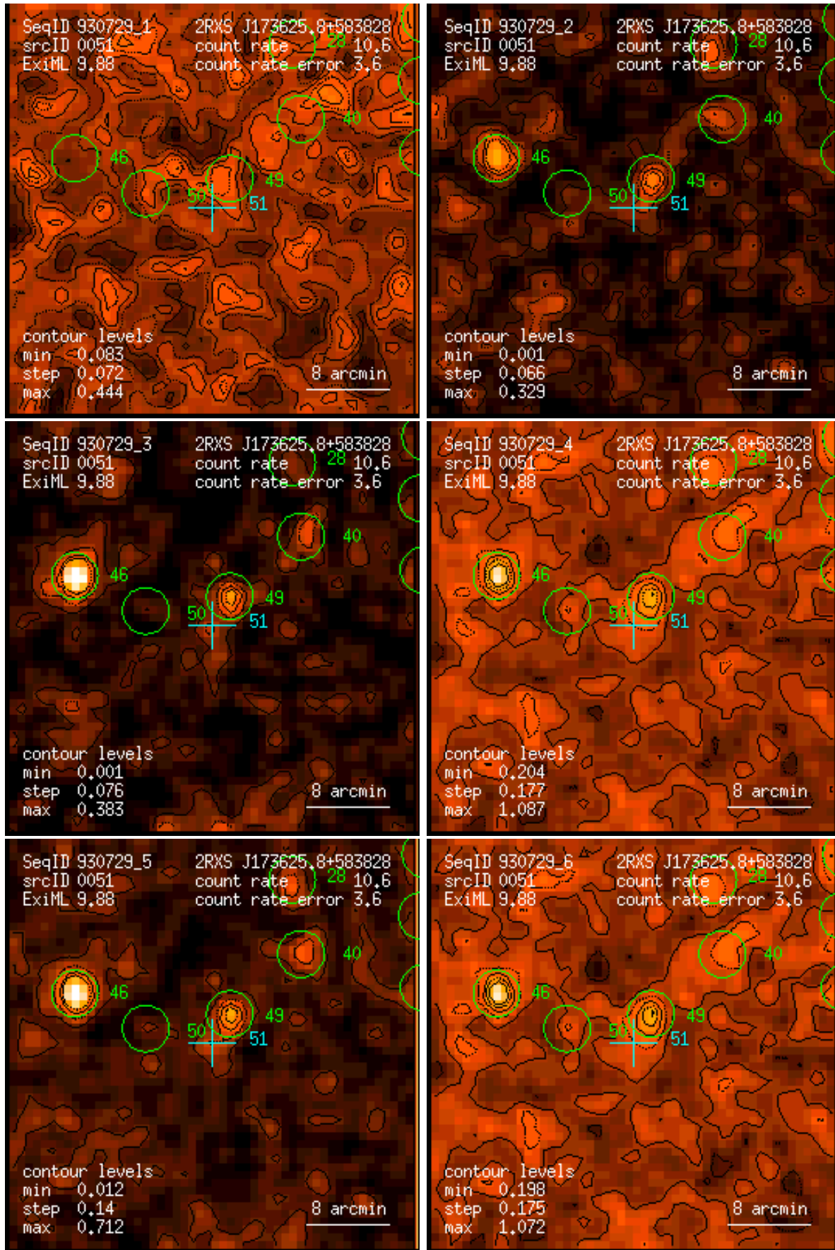
Figure 51: RASS 930729: detection 0051: band rate images, Gaussian filter: (1) PSPC channels 11 – 41, (2) 52 – 90, (3) 91 – 201, (4) 11 – 235, (5) 52 – 201, (6) 11 – 201. Broad band rates in counts/ks. Band rate contour levels in counts/ks/arcmin 2 .
