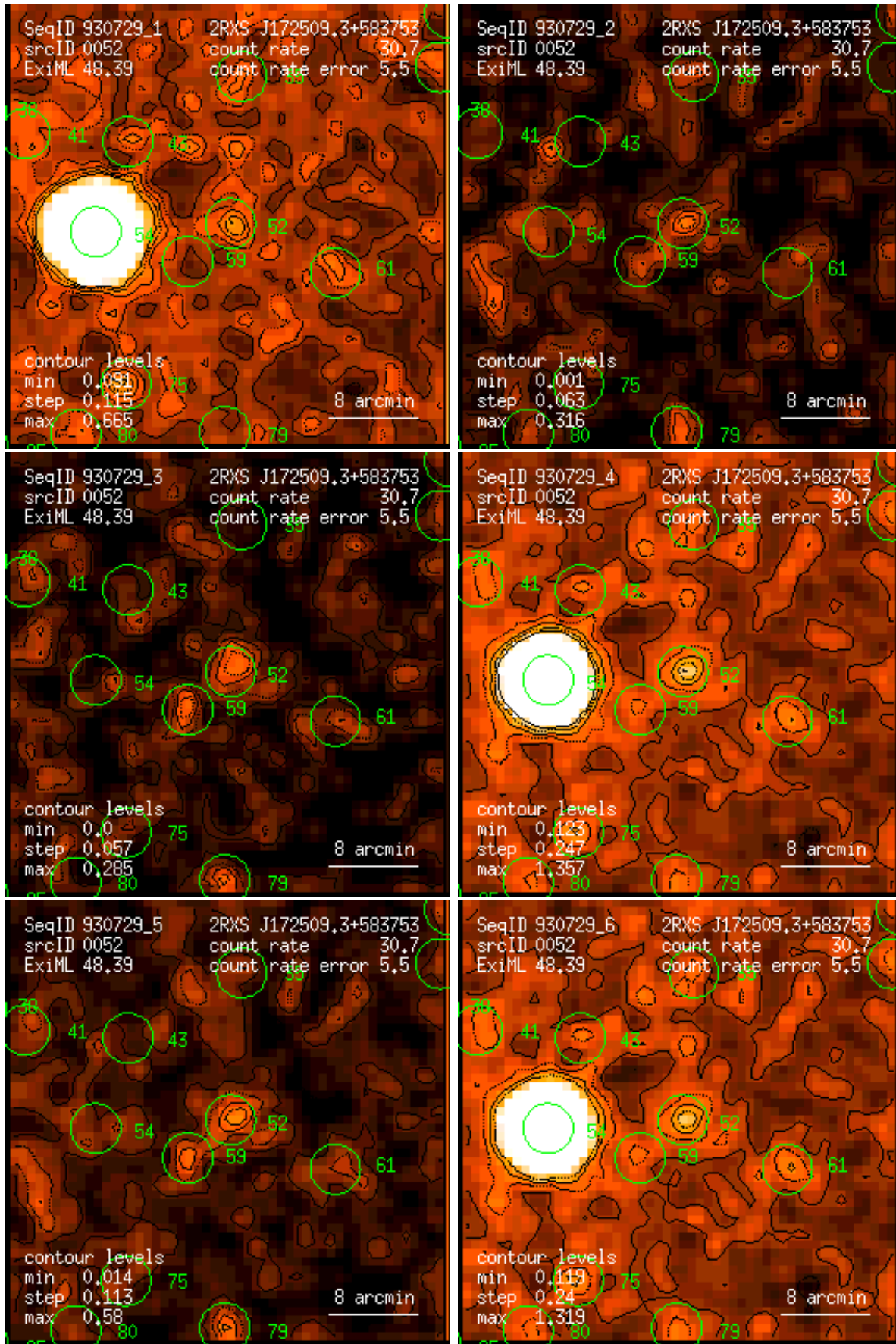
Figure 52: RASS 930729: detection 0052: band rate images, Gaussian filter: (1) PSPC channels 11 – 41, (2) 52 – 90, (3) 91 – 201, (4) 11 – 235, (5) 52 – 201, (6) 11 – 201. Broad band rates in counts/ks. Band rate contour levels in counts/ks/arcmin 2 .
