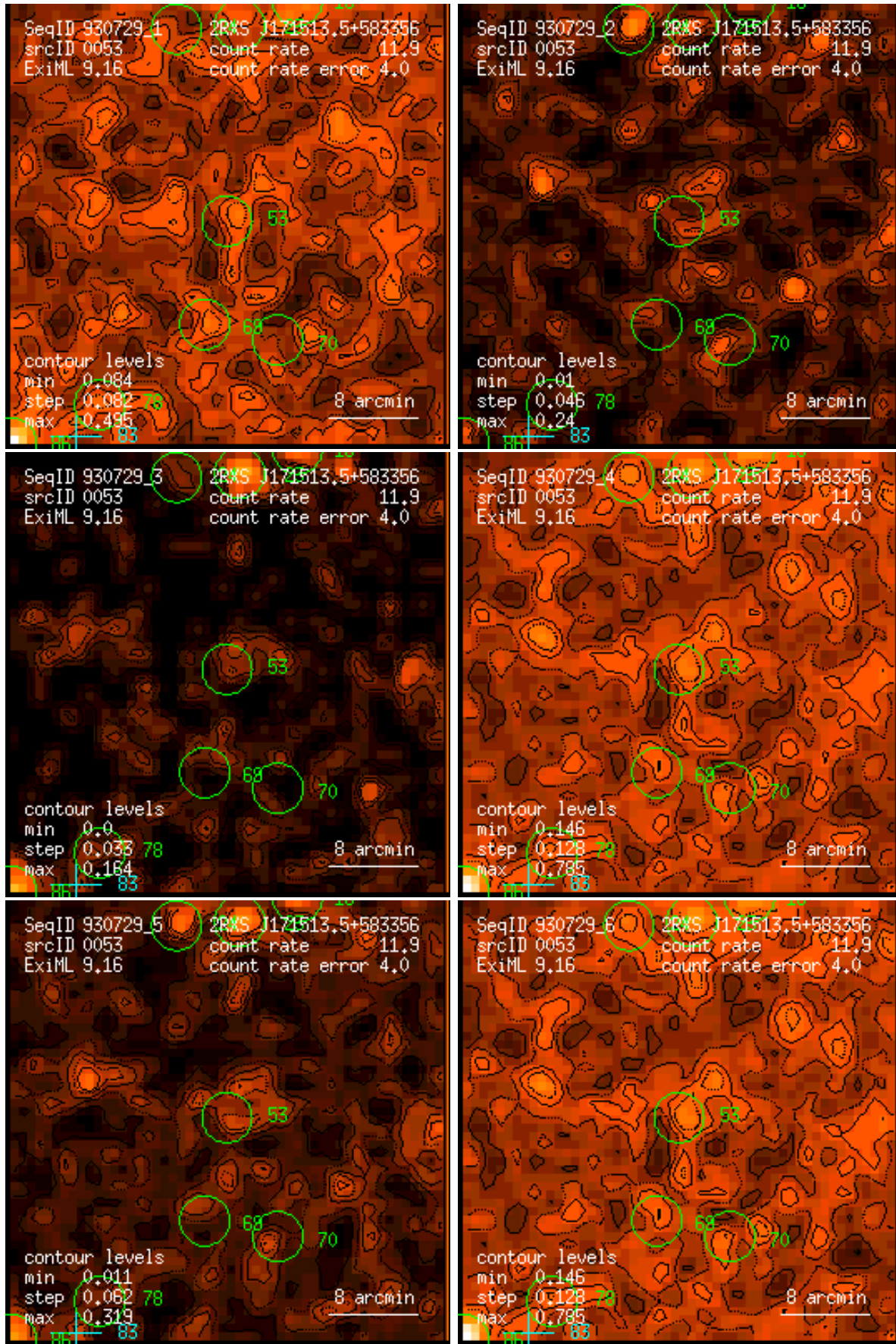
Figure 53: RASS 930729: detection 0053: band rate images, Gaussian filter: (1) PSPC channels 11 – 41, (2) 52 – 90, (3) 91 – 201, (4) 11 – 235, (5) 52 – 201, (6) 11 – 201. Broad band rates in counts/ks. Band rate contour levels in counts/ks/arcmin 2 .
