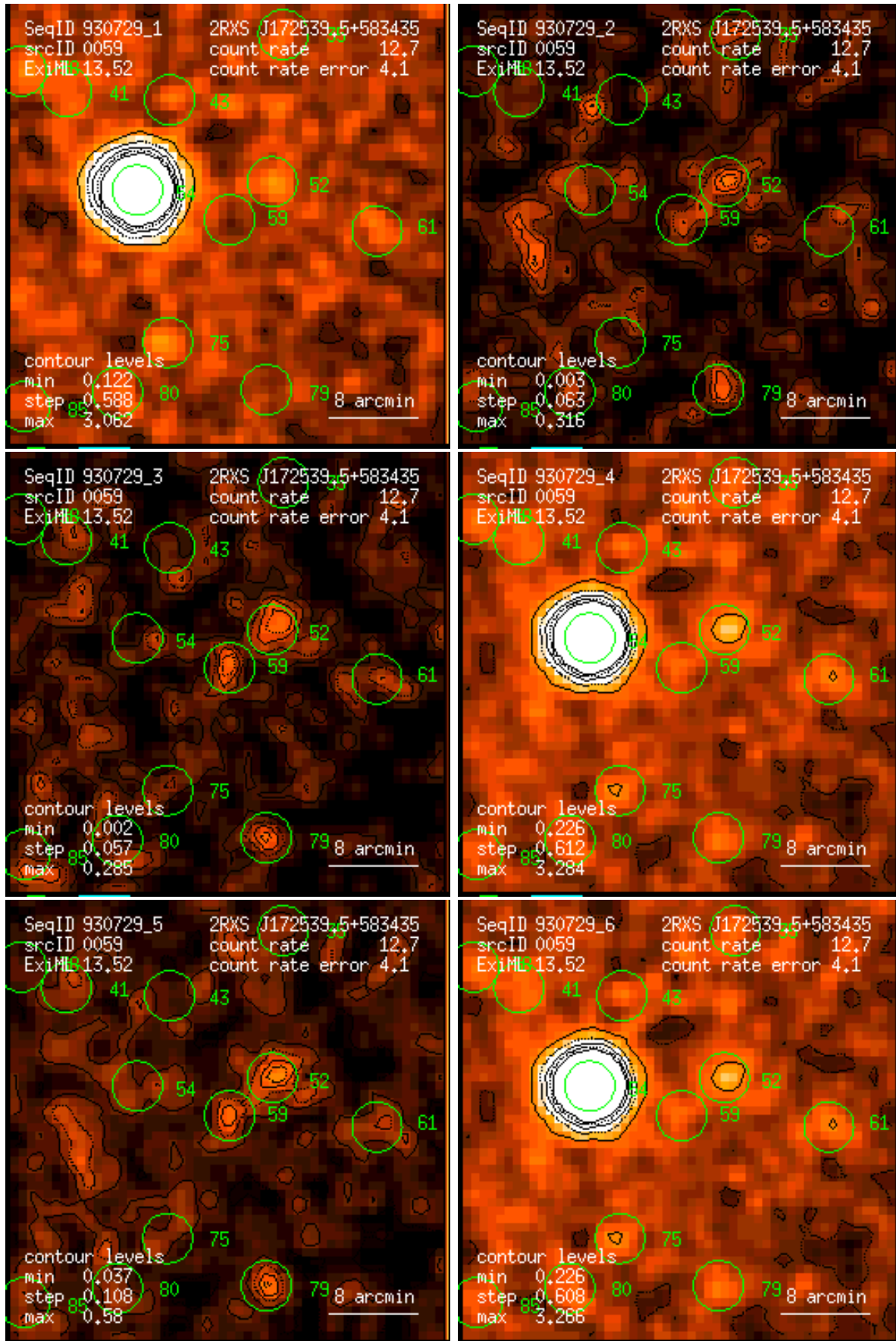
Figure 59: RASS 930729: detection 0059: band rate images, Gaussian filter: (1) PSPC channels 11 – 41, (2) 52 – 90, (3) 91 – 201, (4) 11 – 235, (5) 52 – 201, (6) 11 – 201. Broad band rates in counts/ks. Band rate contour levels in counts/ks/arcmin 2 .
