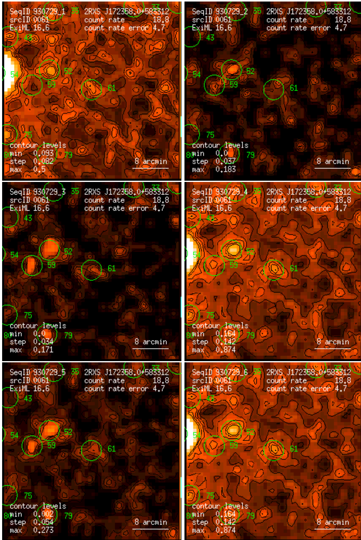
Figure 61: RASS 930729: detection 0061: band rate images, Gaussian filter: (1) PSPC channels 11 – 41, (2) 52 – 90, (3) 91 – 201, (4) 11 – 235, (5) 52 – 201, (6) 11 – 201. Broad band rates in counts/ks. Band rate contour levels in counts/ks/arcmin 2 .
