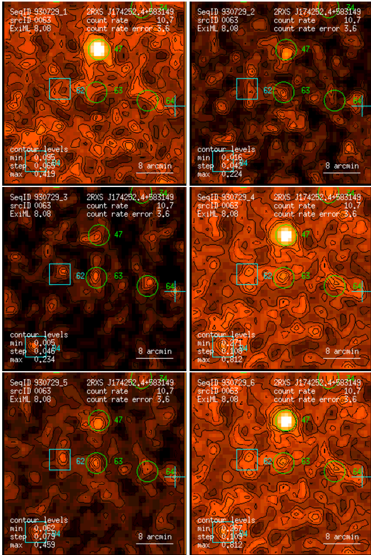
Figure 63: RASS 930729: detection 0063: band rate images, Gaussian filter: (1) PSPC channels 11 – 41, (2) 52 – 90, (3) 91 – 201, (4) 11 – 235, (5) 52 – 201, (6) 11 – 201. Broad band rates in counts/ks. Band rate contour levels in counts/ks/arcmin 2 .
