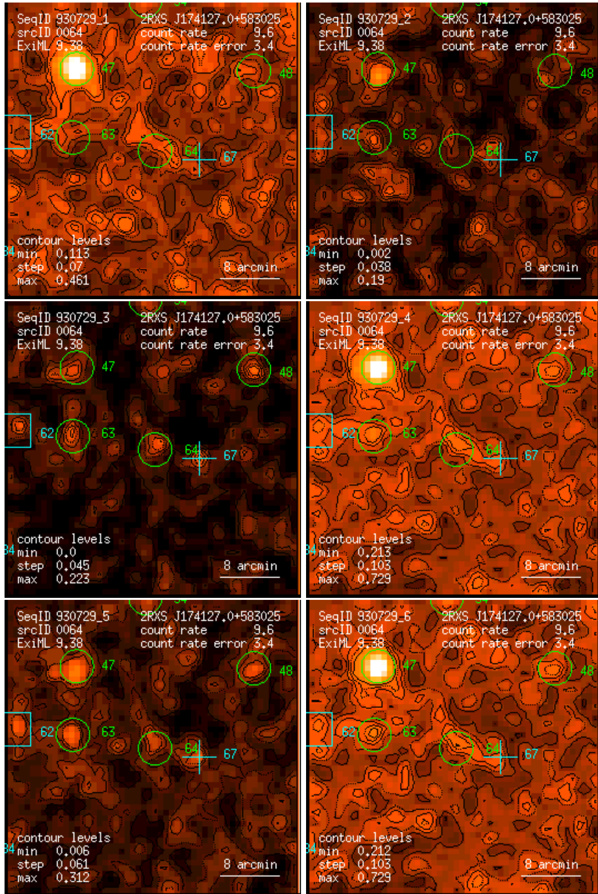
Figure 64: RASS 930729: detection 0064: band rate images, Gaussian filter: (1) PSPC channels 11 – 41, (2) 52 – 90, (3) 91 – 201, (4) 11 – 235, (5) 52 – 201, (6) 11 – 201. Broad band rates in counts/ks. Band rate contour levels in counts/ks/arcmin 2 .
