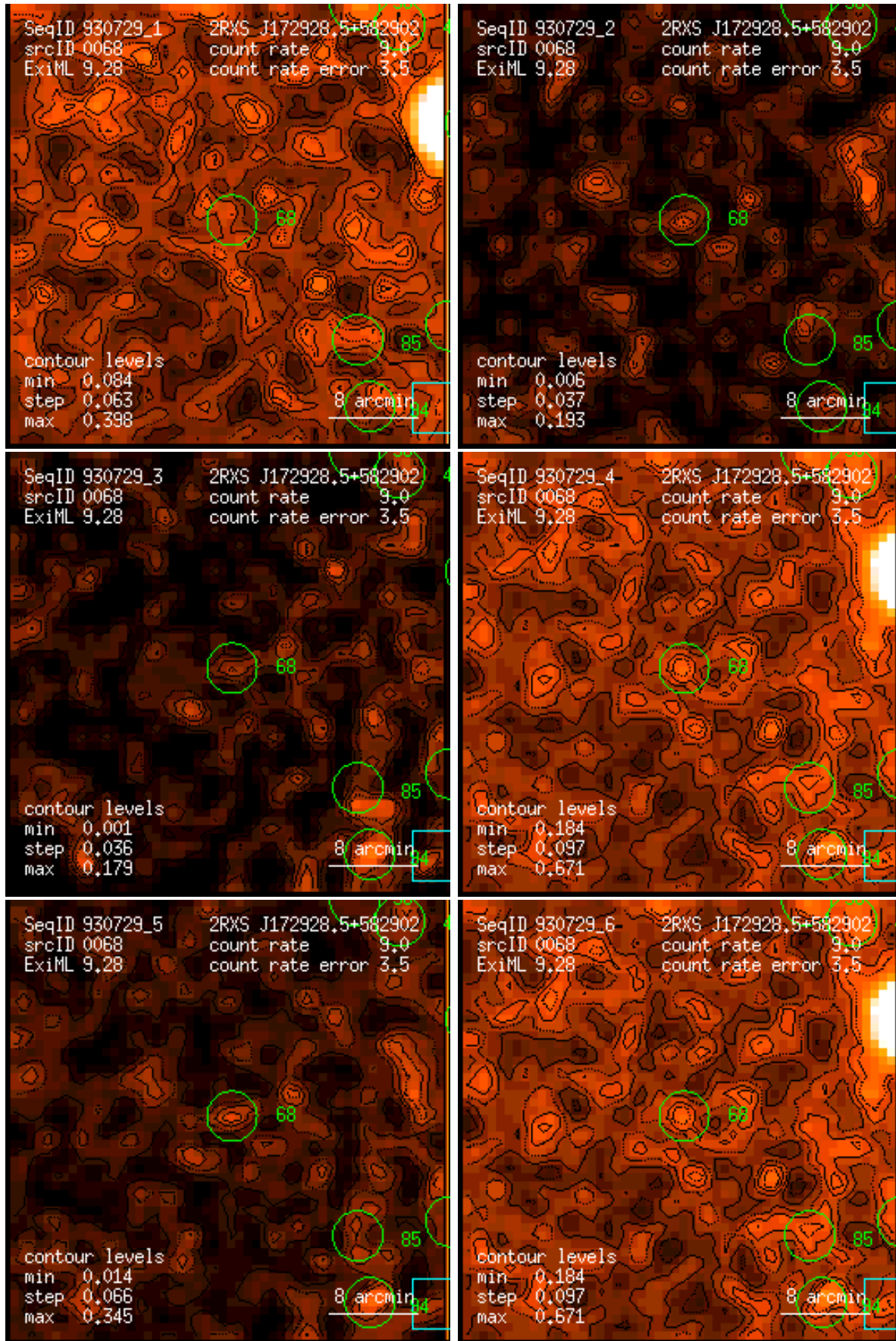
Figure 68: RASS 930729: detection 0068: band rate images, Gaussian filter: (1) PSPC channels 11 – 41, (2) 52 – 90, (3) 91 – 201, (4) 11 – 235, (5) 52 – 201, (6) 11 – 201. Broad band rates in counts/ks. Band rate contour levels in counts/ks/arcmin 2 .
