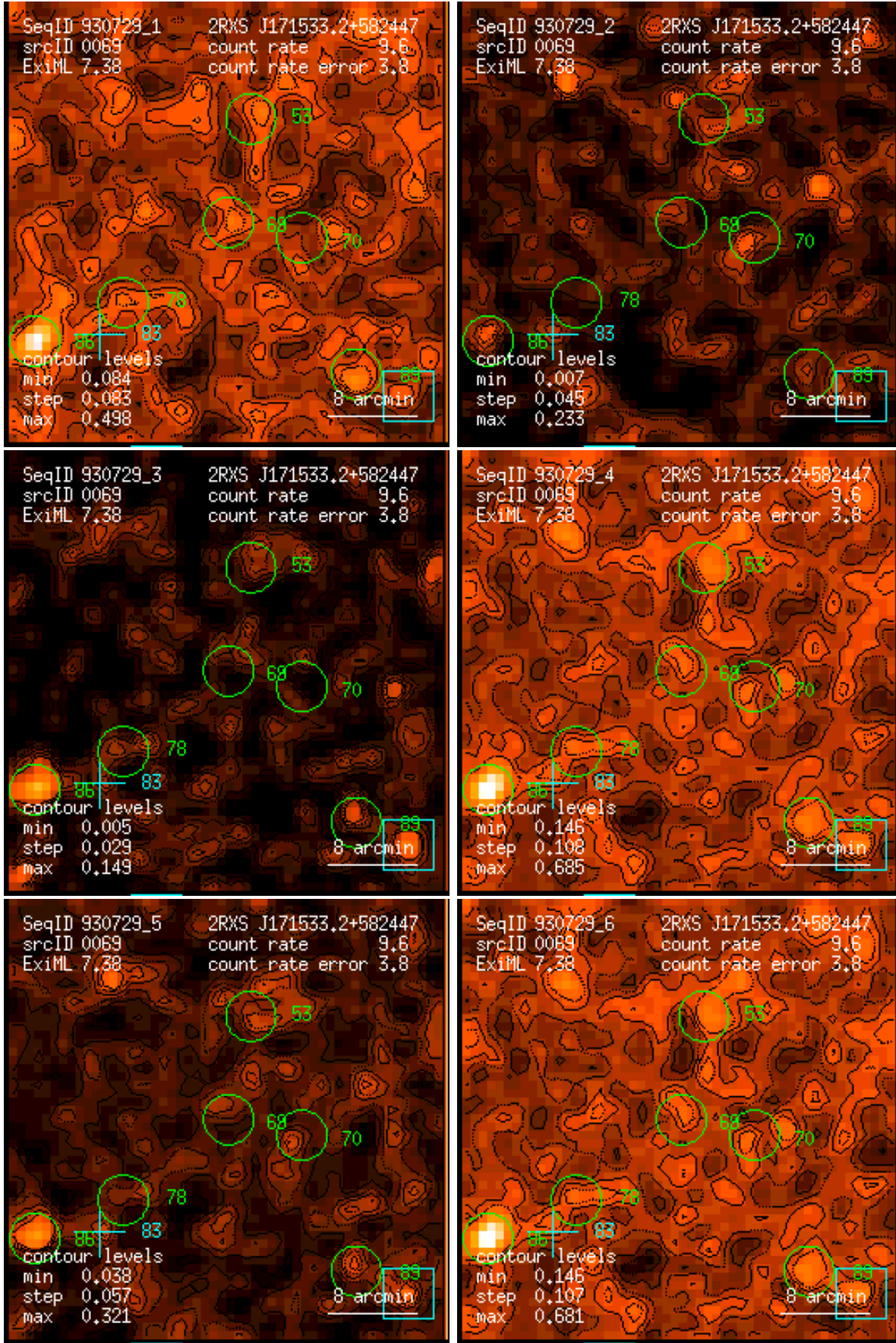
Figure 69: RASS 930729: detection 0069: band rate images, Gaussian filter: (1) PSPC channels 11 – 41, (2) 52 – 90, (3) 91 – 201, (4) 11 – 235, (5) 52 – 201, (6) 11 – 201. Broad band rates in counts/ks. Band rate contour levels in counts/ks/arcmin 2 .
