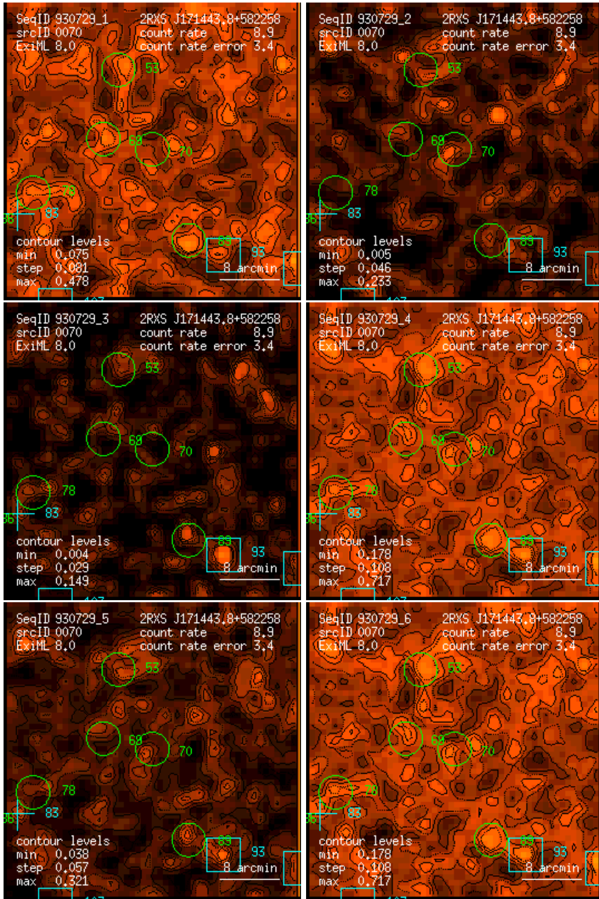
Figure 70: RASS 930729: detection 0070: band rate images, Gaussian filter: (1) PSPC channels 11 – 41, (2) 52 – 90, (3) 91 – 201, (4) 11 – 235, (5) 52 – 201, (6) 11 – 201. Broad band rates in counts/ks. Band rate contour levels in counts/ks/arcmin 2 .
