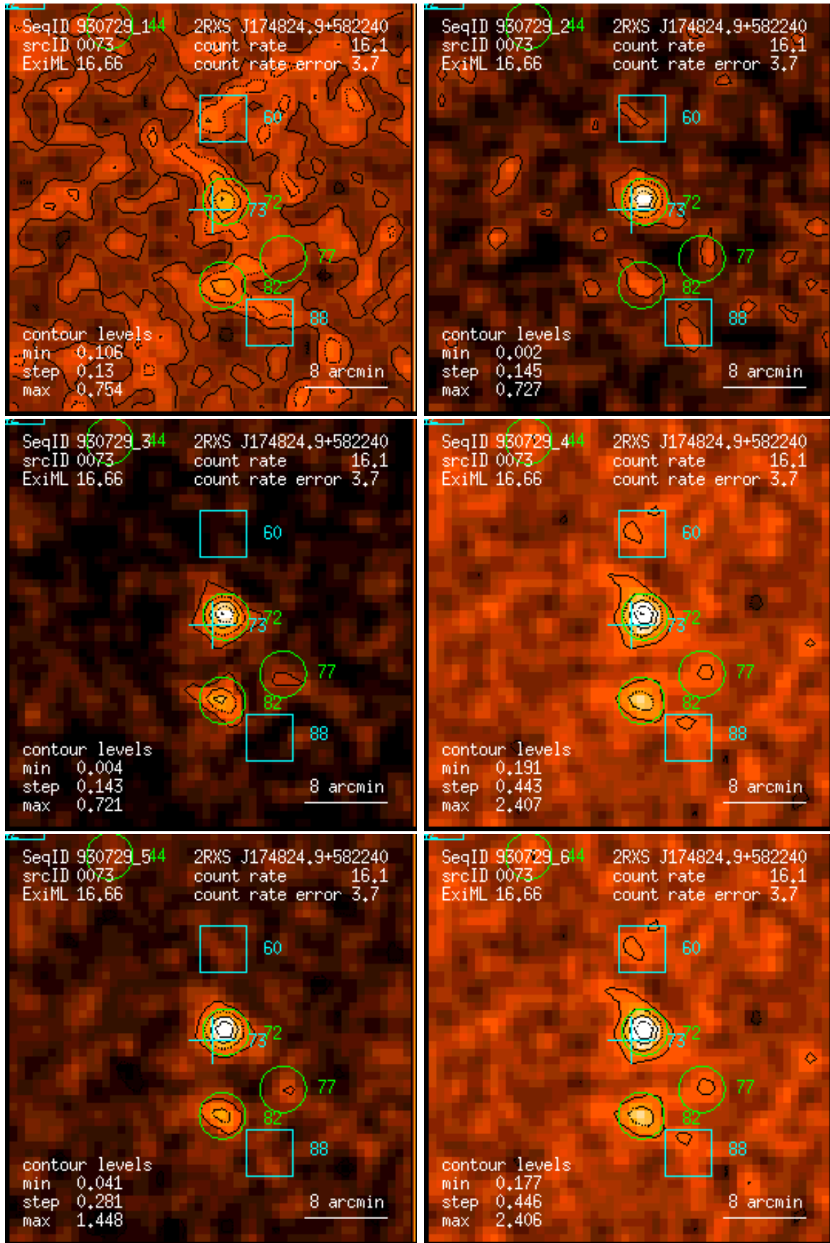
Figure 73: RASS 930729: detection 0073: band rate images, Gaussian filter: (1) PSPC channels 11 – 41, (2) 52 – 90, (3) 91 – 201, (4) 11 – 235, (5) 52 – 201, (6) 11 – 201. Broad band rates in counts/ks. Band rate contour levels in counts/ks/arcmin 2 .
