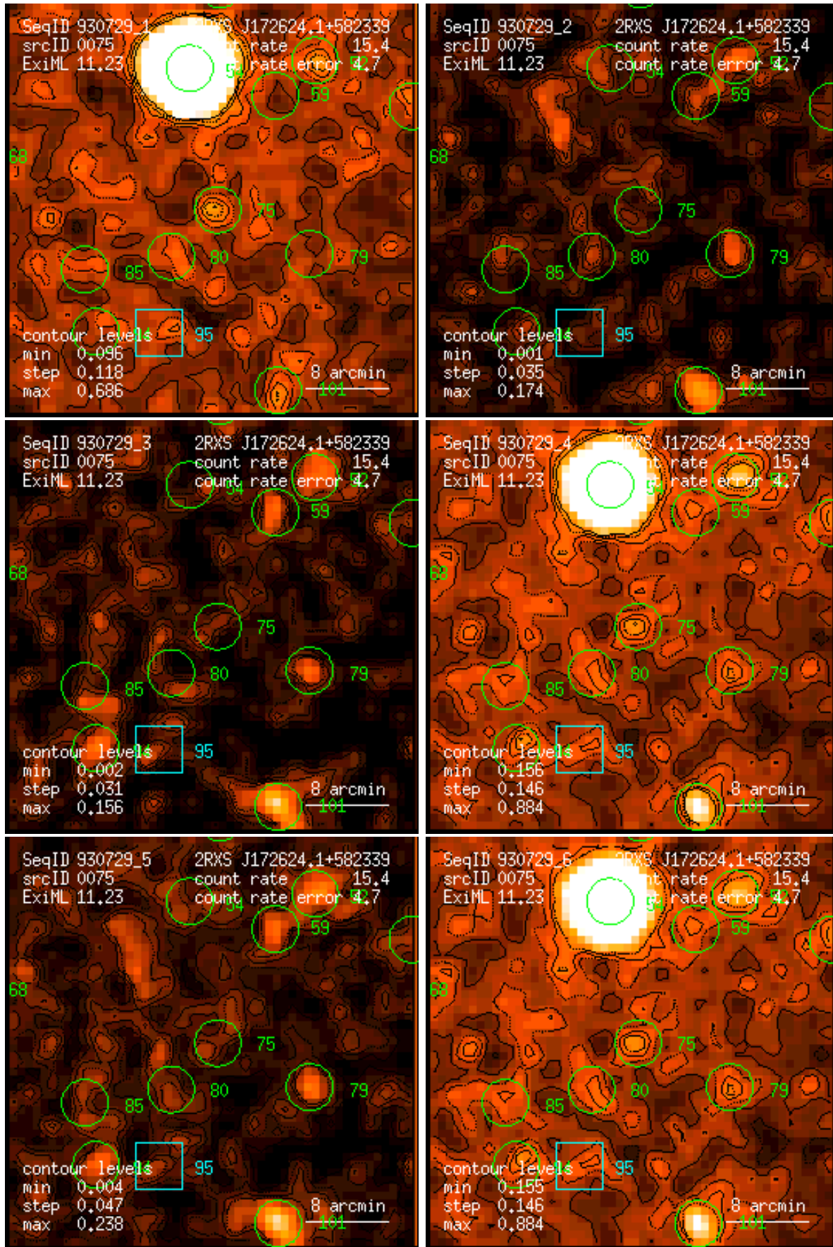
Figure 75: RASS 930729: detection 0075: band rate images, Gaussian filter: (1) PSPC channels 11 – 41, (2) 52 – 90, (3) 91 – 201, (4) 11 – 235, (5) 52 – 201, (6) 11 – 201. Broad band rates in counts/ks. Band rate contour levels in counts/ks/arcmin 2 .
