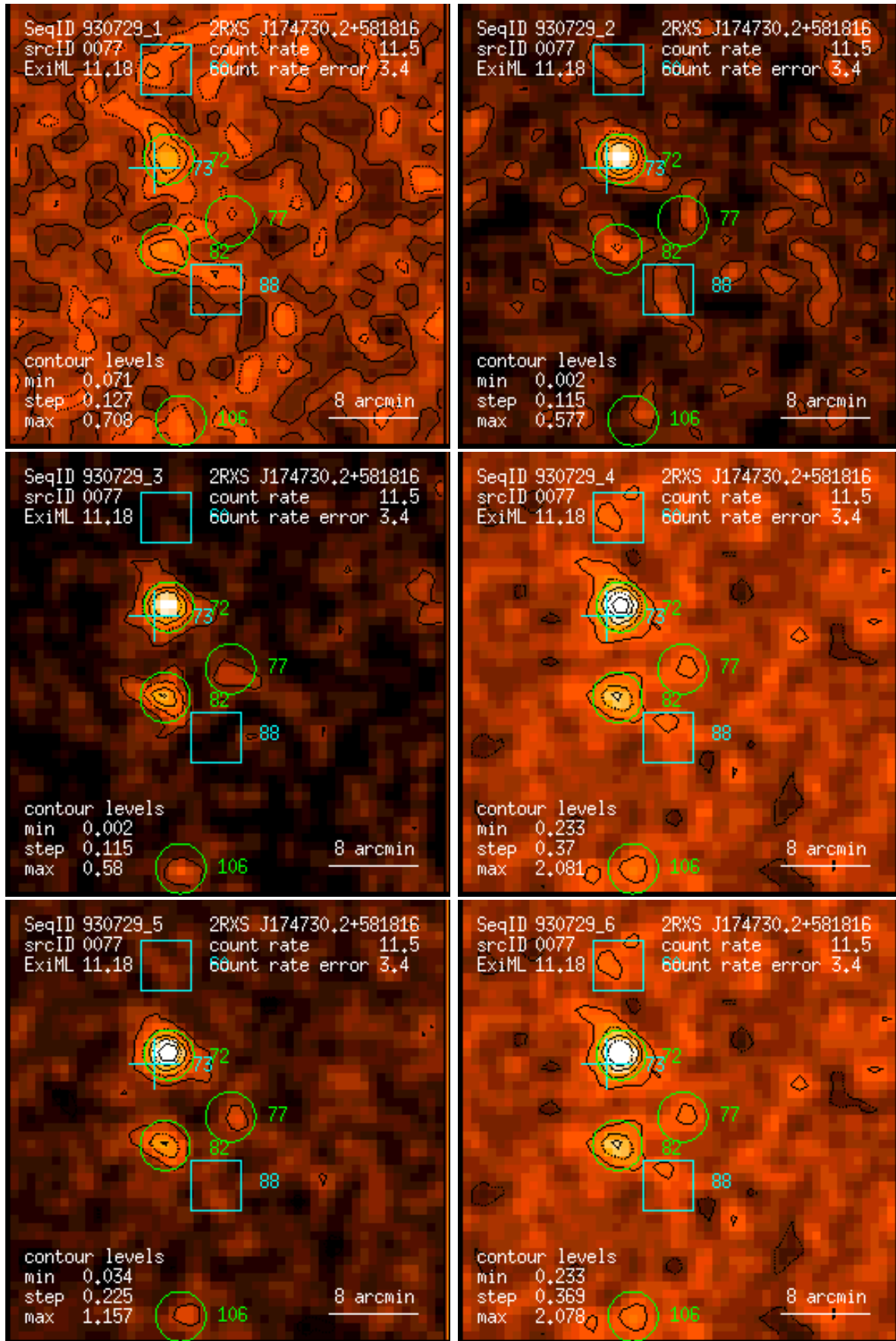
Figure 77: RASS 930729: detection 0077: band rate images, Gaussian filter: (1) PSPC channels 11 – 41, (2) 52 – 90, (3) 91 – 201, (4) 11 – 235, (5) 52 – 201, (6) 11 – 201. Broad band rates in counts/ks. Band rate contour levels in counts/ks/arcmin 2 .
