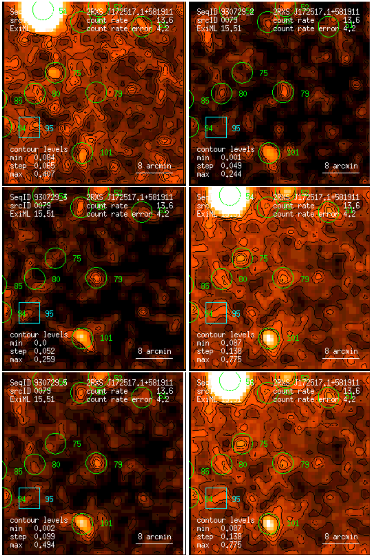
Figure 79: RASS 930729: detection 0079: band rate images, Gaussian filter: (1) PSPC channels 11 – 41, (2) 52 – 90, (3) 91 – 201, (4) 11 – 235, (5) 52 – 201, (6) 11 – 201. Broad band rates in counts/ks. Band rate contour levels in counts/ks/arcmin 2 .
