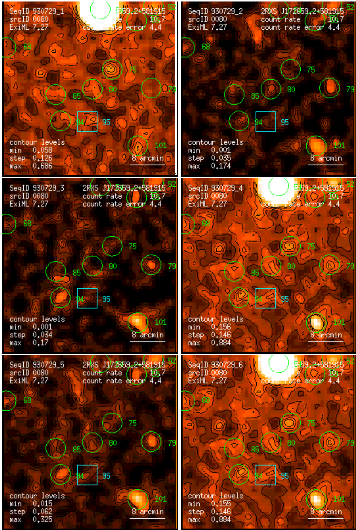
Figure 80: RASS 930729: detection 0080: band rate images, Gaussian filter: (1) PSPC channels 11 – 41, (2) 52 – 90, (3) 91 – 201, (4) 11 – 235, (5) 52 – 201, (6) 11 – 201. Broad band rates in counts/ks. Band rate contour levels in counts/ks/arcmin 2 .
