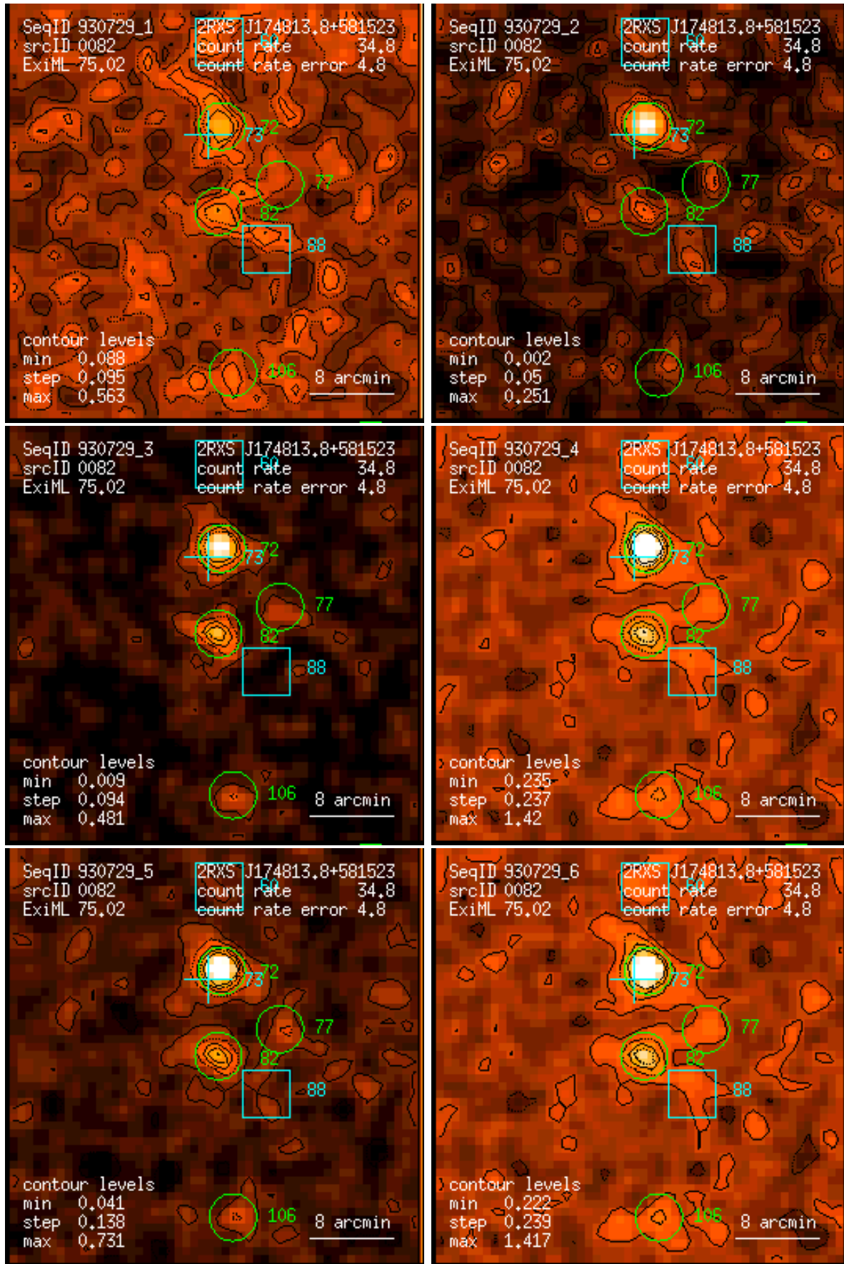
Figure 82: RASS 930729: detection 0082: band rate images, Gaussian filter: (1) PSPC channels 11 – 41, (2) 52 – 90, (3) 91 – 201, (4) 11 – 235, (5) 52 – 201, (6) 11 – 201. Broad band rates in counts/ks. Band rate contour levels in counts/ks/arcmin 2 .
