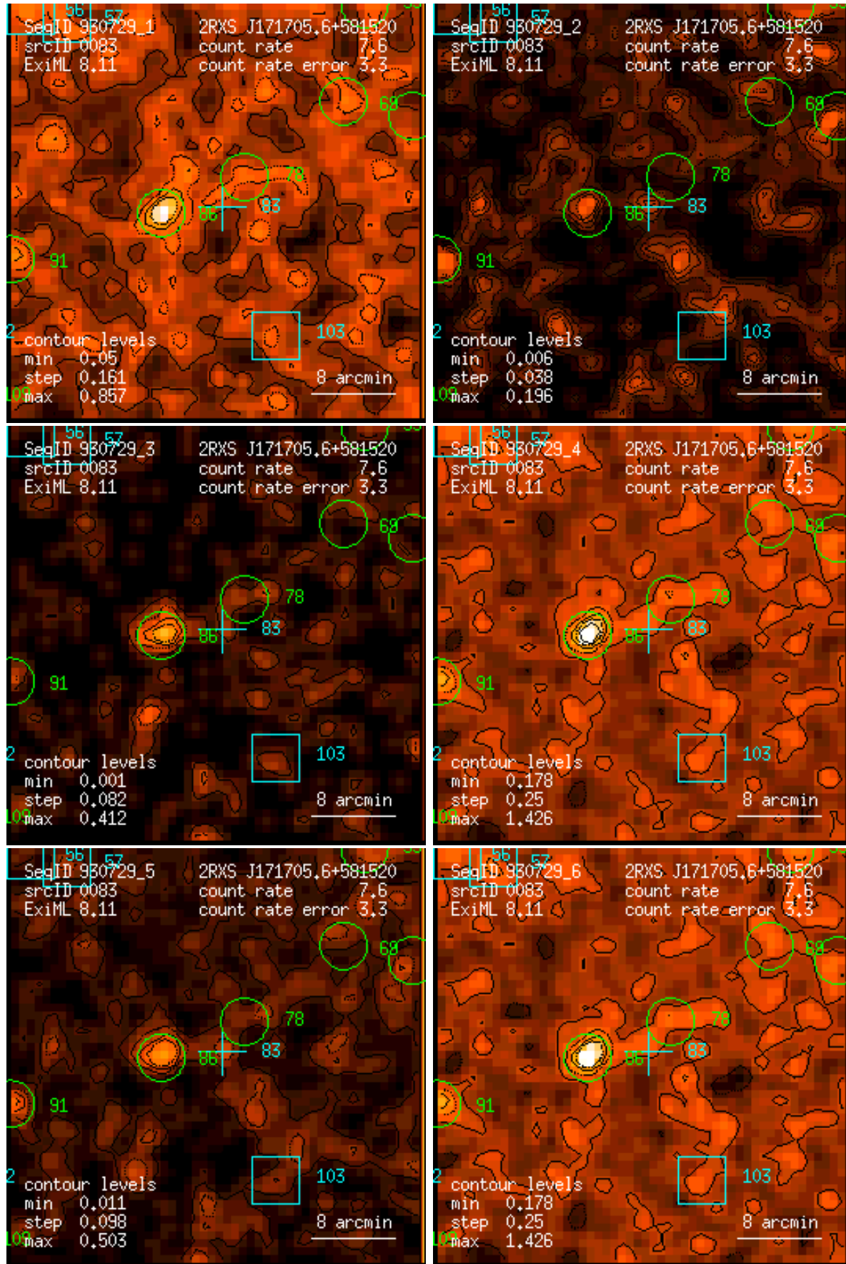
Figure 83: RASS 930729: detection 0083: band rate images, Gaussian filter: (1) PSPC channels 11 – 41, (2) 52 – 90, (3) 91 – 201, (4) 11 – 235, (5) 52 – 201, (6) 11 – 201. Broad band rates in counts/ks. Band rate contour levels in counts/ks/arcmin 2 .
