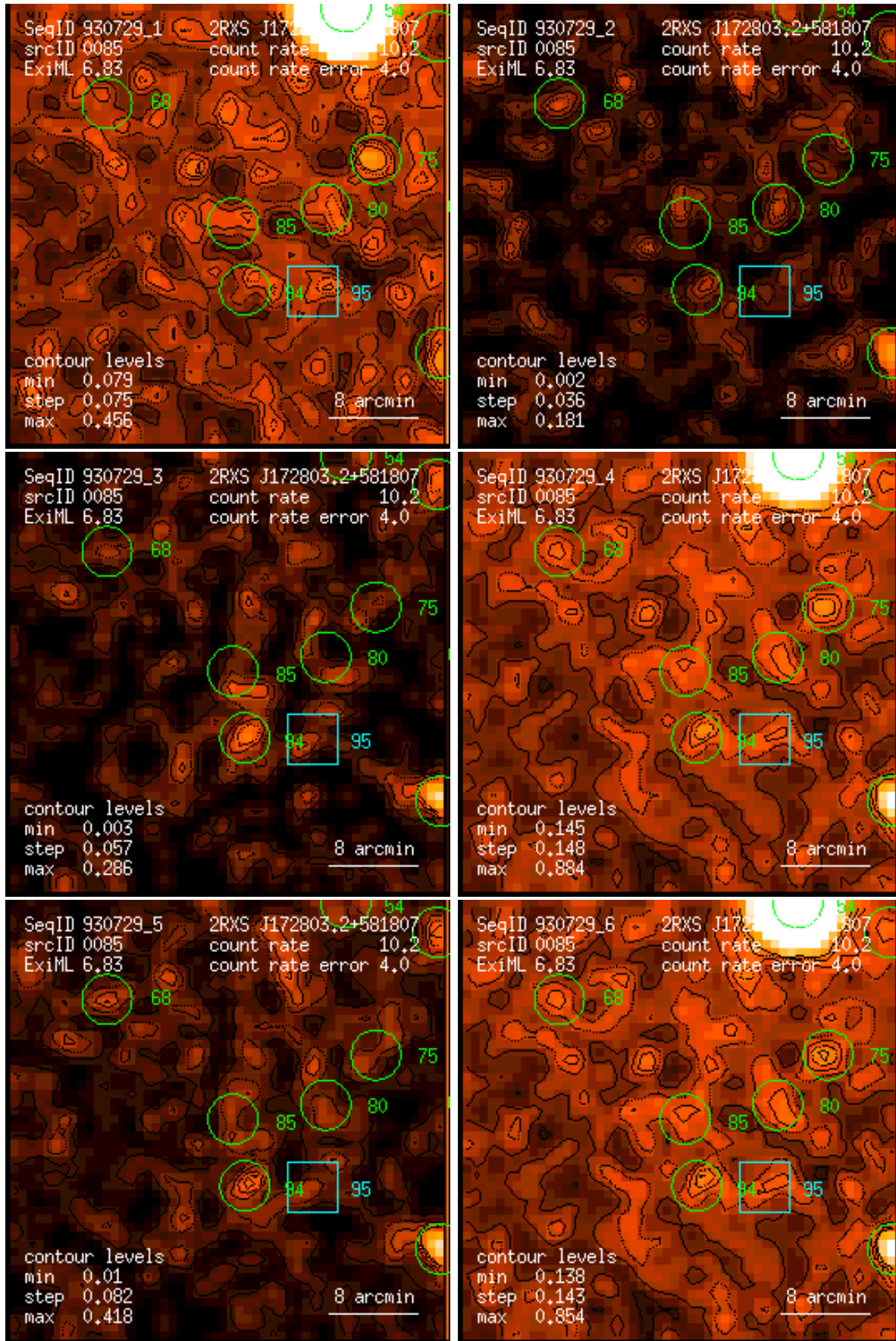
Figure 85: RASS 930729: detection 0085: band rate images, Gaussian filter: (1) PSPC channels 11 – 41, (2) 52 – 90, (3) 91 – 201, (4) 11 – 235, (5) 52 – 201, (6) 11 – 201. Broad band rates in counts/ks. Band rate contour levels in counts/ks/arcmin 2 .
