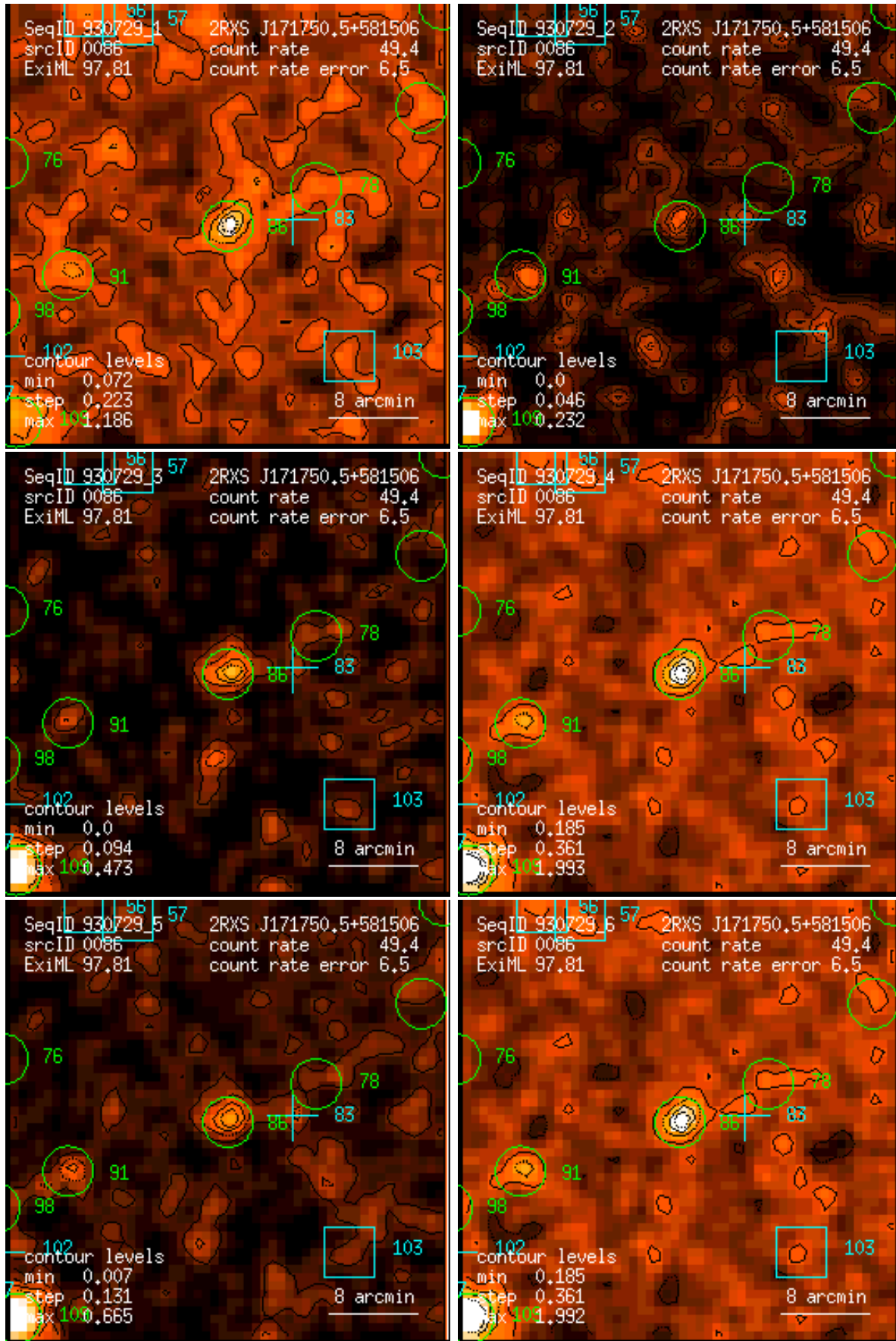
Figure 86: RASS 930729: detection 0086: band rate images, Gaussian filter: (1) PSPC channels 11 – 41, (2) 52 – 90, (3) 91 – 201, (4) 11 – 235, (5) 52 – 201, (6) 11 – 201. Broad band rates in counts/ks. Band rate contour levels in counts/ks/arcmin 2 .
