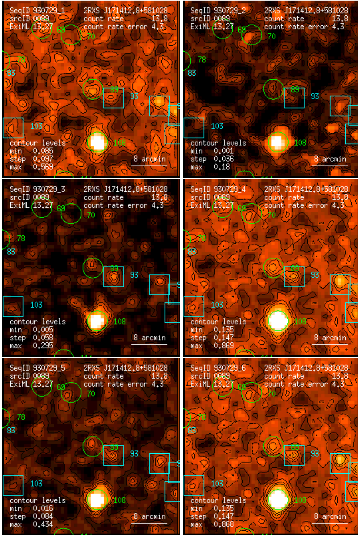
Figure 89: RASS 930729: detection 0089: band rate images, Gaussian filter: (1) PSPC channels 11 – 41, (2) 52 – 90, (3) 91 – 201, (4) 11 – 235, (5) 52 – 201, (6) 11 – 201. Broad band rates in counts/ks. Band rate contour levels in counts/ks/arcmin 2 .
