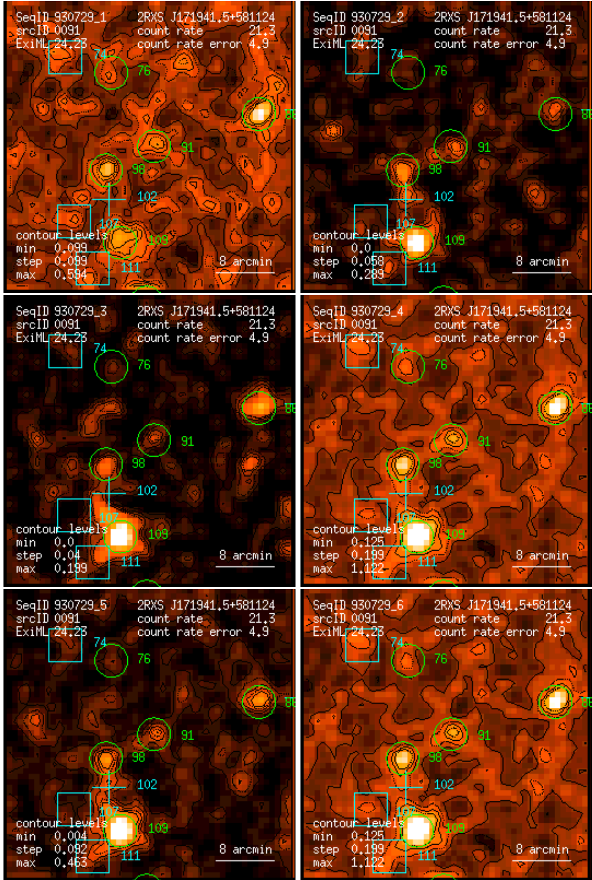
Figure 91: RASS 930729: detection 0091: band rate images, Gaussian filter: (1) PSPC channels 11 – 41, (2) 52 – 90, (3) 91 – 201, (4) 11 – 235, (5) 52 – 201, (6) 11 – 201. Broad band rates in counts/ks. Band rate contour levels in counts/ks/arcmin 2 .
