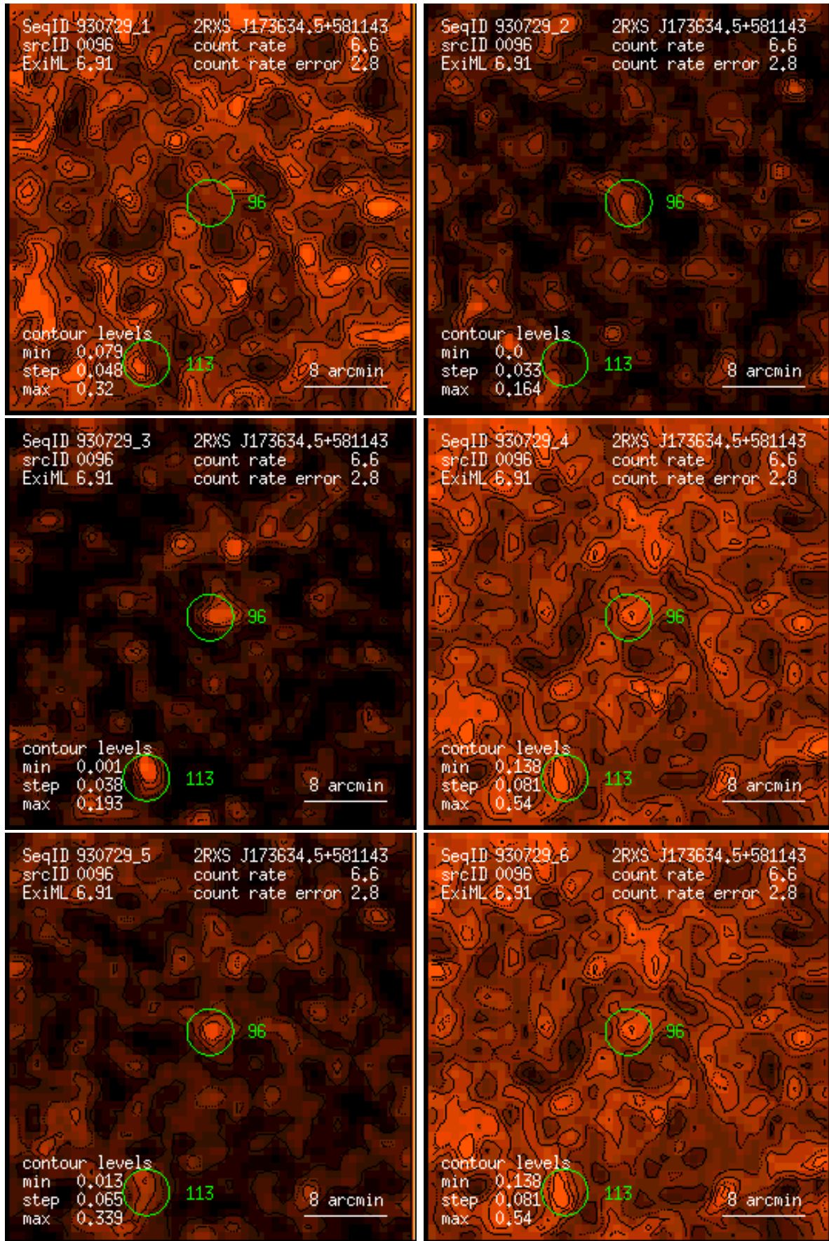
Figure 96: RASS 930729: detection 0096: band rate images, Gaussian filter: (1) PSPC channels 11 – 41, (2) 52 – 90, (3) 91 – 201, (4) 11 – 235, (5) 52 – 201, (6) 11 – 201. Broad band rates in counts/ks. Band rate contour levels in counts/ks/arcmin 2 .
