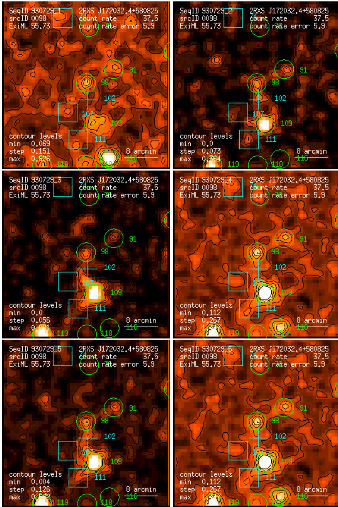
Figure 98: RASS 930729: detection 0098: band rate images, Gaussian filter: (1) PSPC channels 11 – 41, (2) 52 – 90, (3) 91 – 201, (4) 11 – 235, (5) 52 – 201, (6) 11 – 201. Broad band rates in counts/ks. Band rate contour levels in counts/ks/arcmin 2 .
