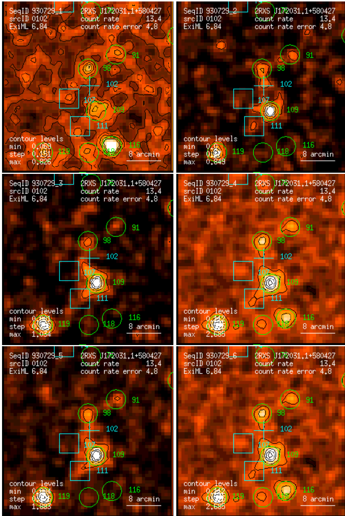
Figure 102: RASS 930729: detection 0102: band rate images, Gaussian filter: (1) PSPC channels 11 – 41, (2) 52 – 90, (3) 91 – 201, (4) 11 – 235, (5) 52 – 201, (6) 11 – 201. Broad band rates in counts/ks. Band rate contour levels in counts/ks/arcmin 2 .
