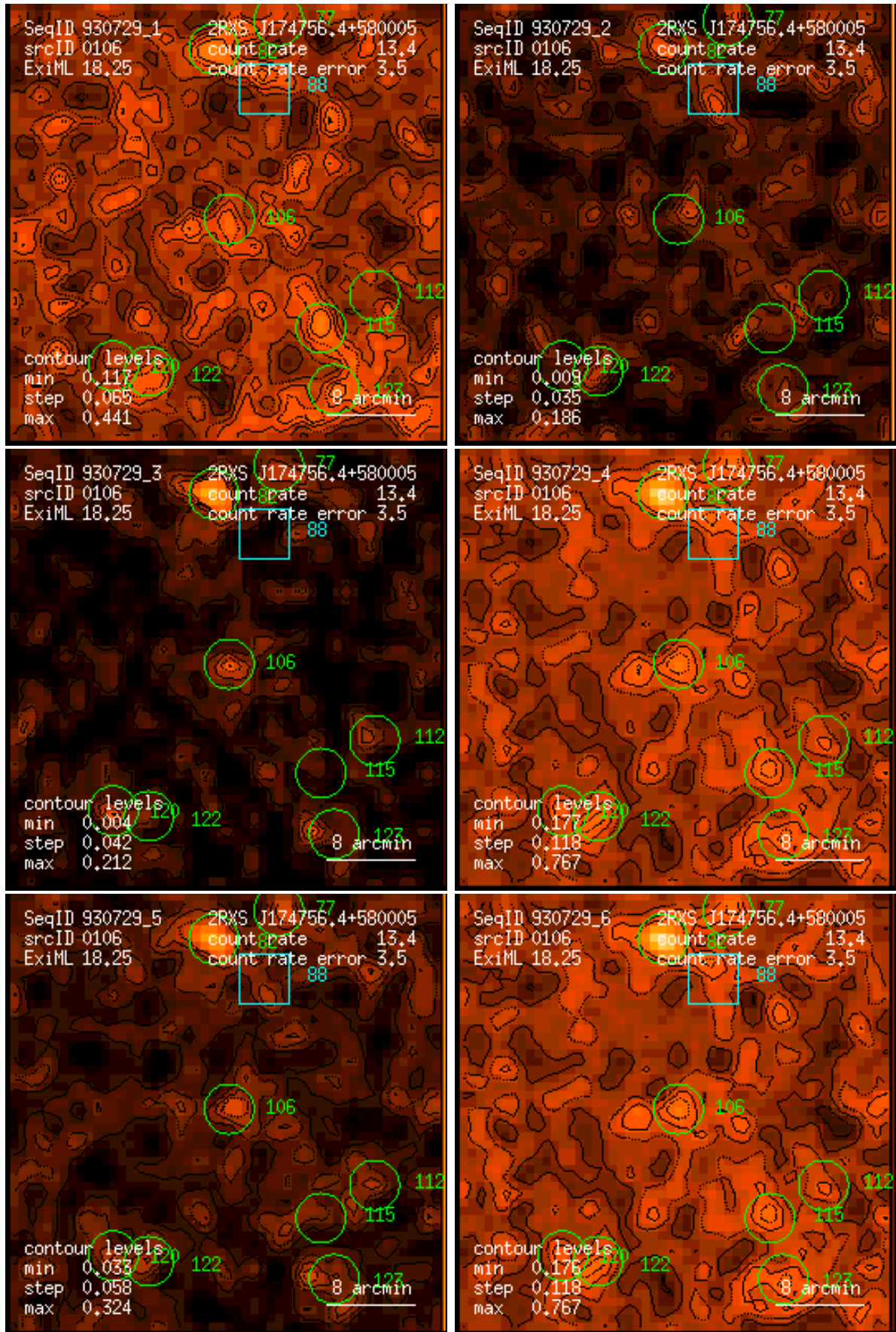
Figure 106: RASS 930729: detection 0106: band rate images, Gaussian filter: (1) PSPC channels 11 – 41, (2) 52 – 90, (3) 91 – 201, (4) 11 – 235, (5) 52 – 201, (6) 11 – 201. Broad band rates in counts/ks. Band rate contour levels in counts/ks/arcmin 2 .
