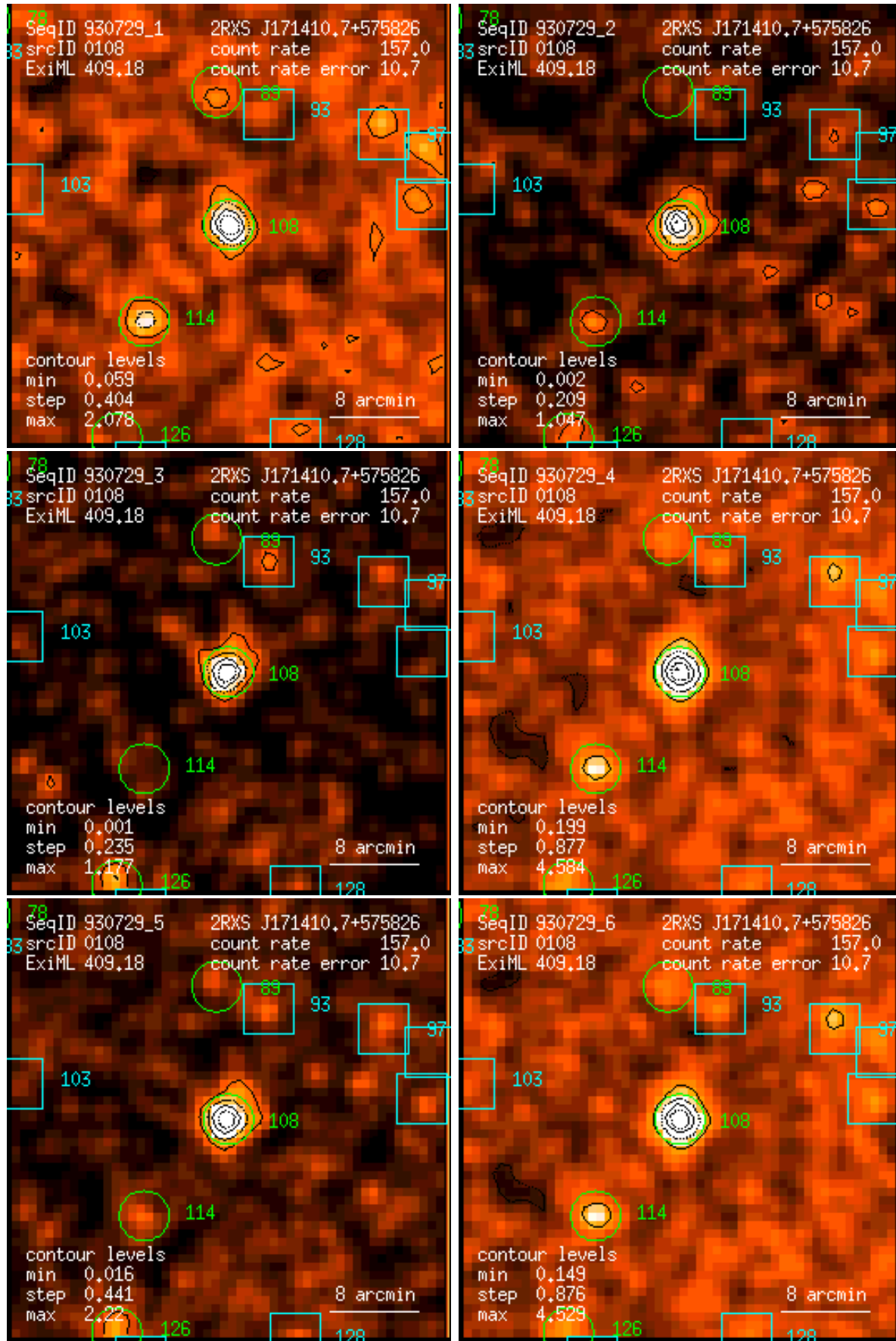
Figure 108: RASS 930729: detection 0108: band rate images, Gaussian filter: (1) PSPC channels 11 – 41, (2) 52 – 90, (3) 91 – 201, (4) 11 – 235, (5) 52 – 201, (6) 11 – 201. Broad band rates in counts/ks. Band rate contour levels in counts/ks/arcmin 2 .
