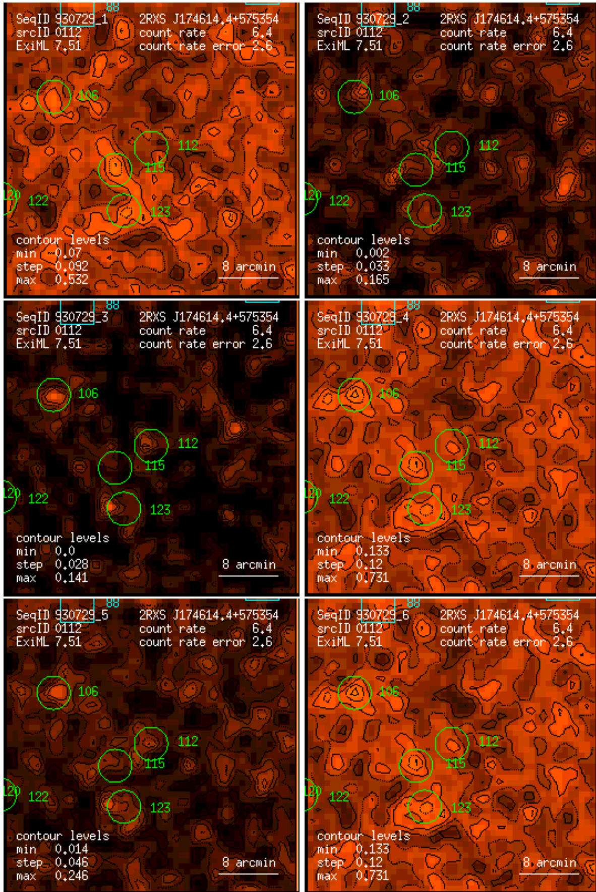
Figure 112: RASS 930729: detection 0112: band rate images, Gaussian filter: (1) PSPC channels 11 – 41, (2) 52 – 90, (3) 91 – 201, (4) 11 – 235, (5) 52 – 201, (6) 11 – 201. Broad band rates in counts/ks. Band rate contour levels in counts/ks/arcmin 2 .
