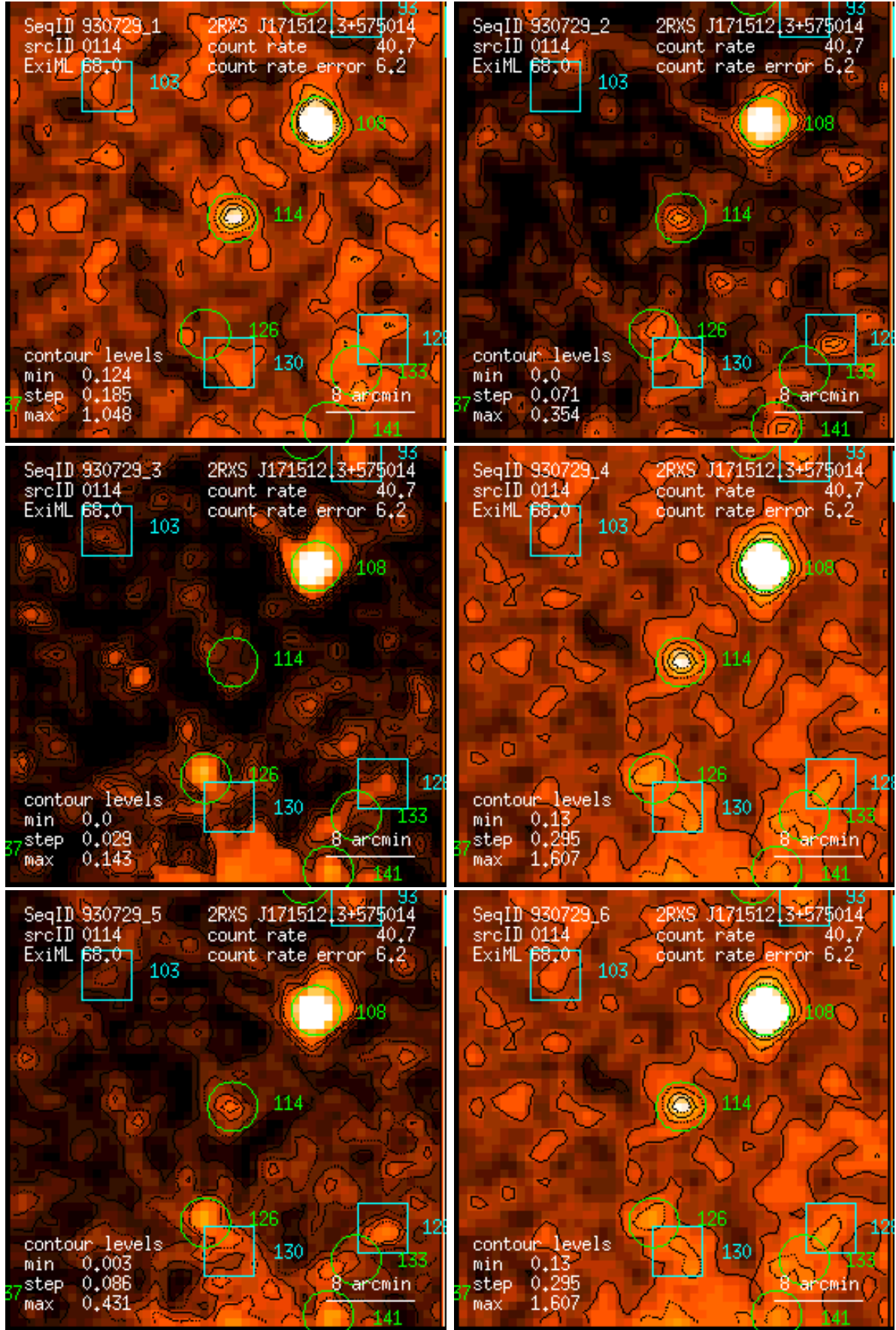
Figure 114: RASS 930729: detection 0114: band rate images, Gaussian filter: (1) PSPC channels 11 – 41, (2) 52 – 90, (3) 91 – 201, (4) 11 – 235, (5) 52 – 201, (6) 11 – 201. Broad band rates in counts/ks. Band rate contour levels in counts/ks/arcmin 2 .
