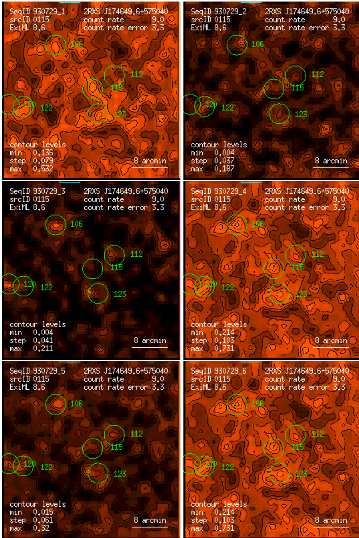
Figure 115: RASS 930729: detection 0115: band rate images, Gaussian filter: (1) PSPC channels 11 – 41, (2) 52 – 90, (3) 91 – 201, (4) 11 – 235, (5) 52 – 201, (6) 11 – 201. Broad band rates in counts/ks. Band rate contour levels in counts/ks/arcmin 2 .
