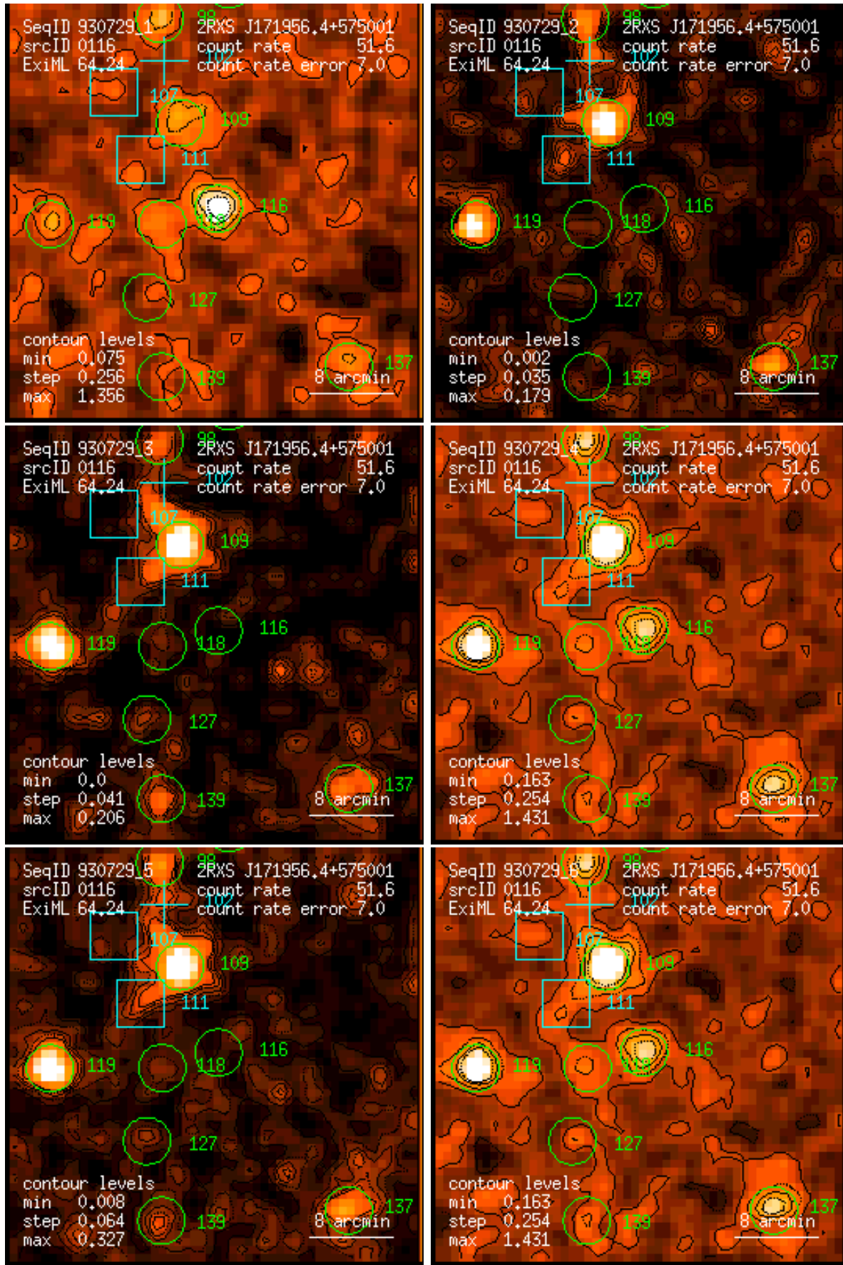
Figure 116: RASS 930729: detection 0116: band rate images, Gaussian filter: (1) PSPC channels 11 – 41, (2) 52 – 90, (3) 91 – 201, (4) 11 – 235, (5) 52 – 201, (6) 11 – 201. Broad band rates in counts/ks. Band rate contour levels in counts/ks/arcmin 2 .
