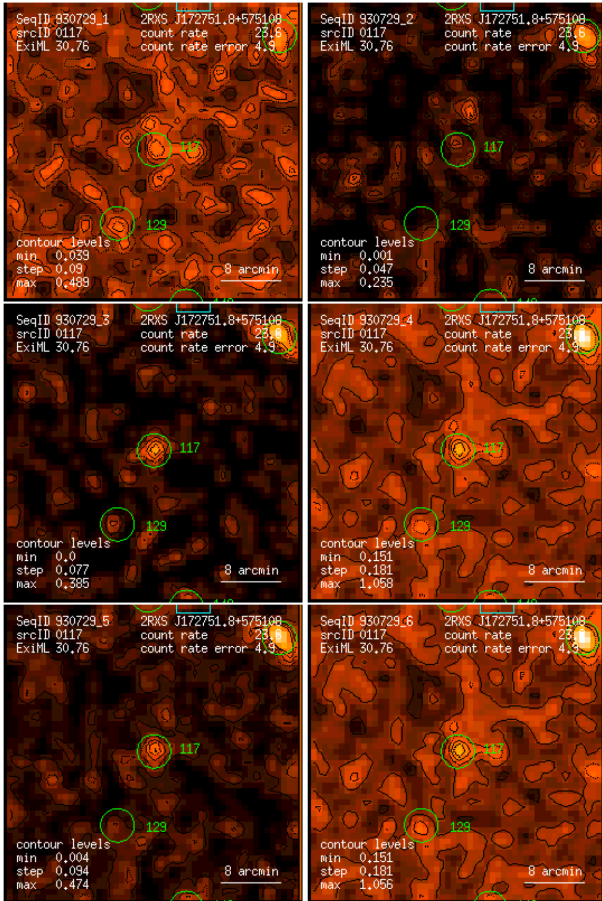
Figure 117: RASS 930729: detection 0117: band rate images, Gaussian filter: (1) PSPC channels 11 – 41, (2) 52 – 90, (3) 91 – 201, (4) 11 – 235, (5) 52 – 201, (6) 11 – 201. Broad band rates in counts/ks. Band rate contour levels in counts/ks/arcmin 2 .
