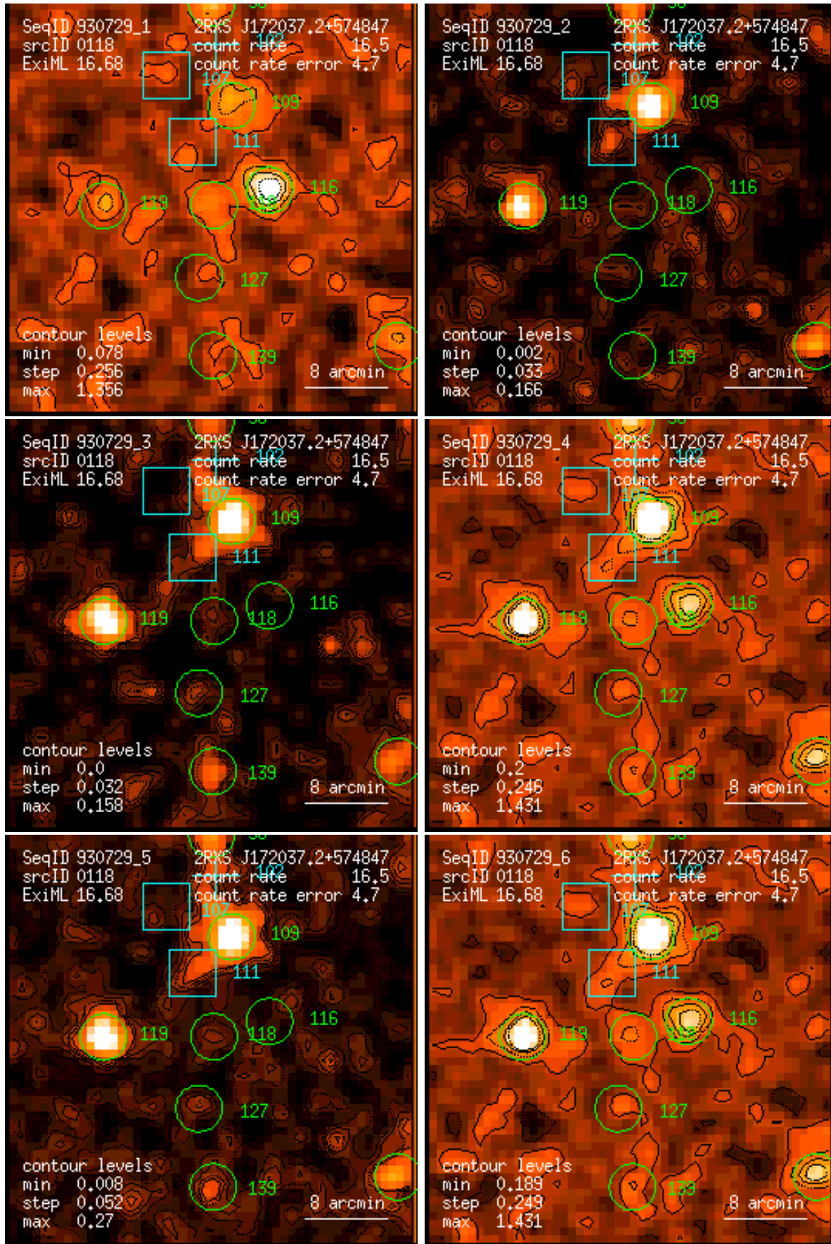
Figure 118: RASS 930729: detection 0118: band rate images, Gaussian filter: (1) PSPC channels 11 – 41, (2) 52 – 90, (3) 91 – 201, (4) 11 – 235, (5) 52 – 201, (6) 11 – 201. Broad band rates in counts/ks. Band rate contour levels in counts/ks/arcmin 2 .
